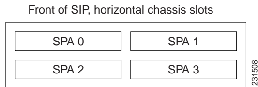
Figure 2-2 Cisco ASR 1000 Series SIP SPA Numbering
