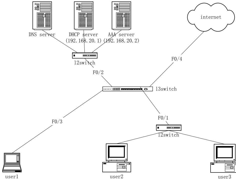
Figure 3-4 Network topology
