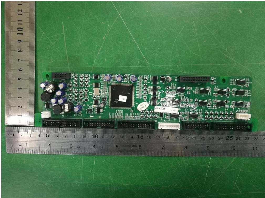
Figure 8: PCB component view
