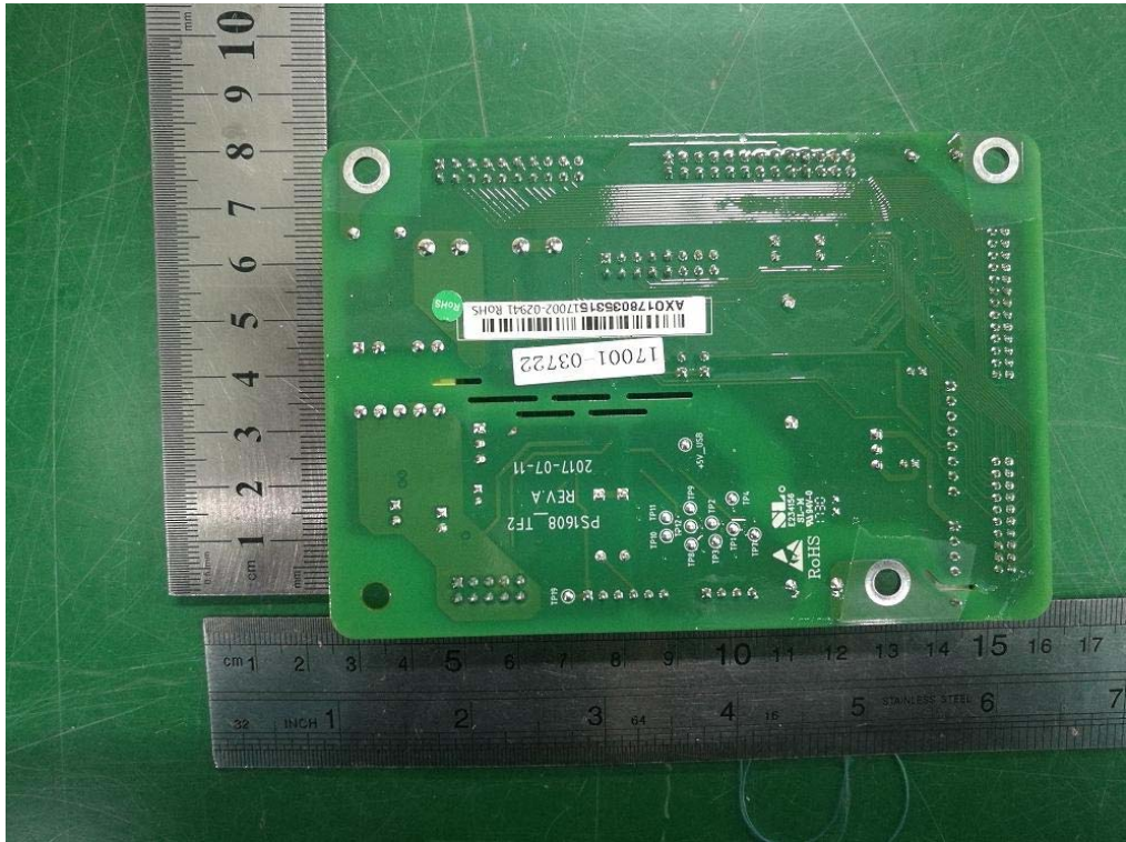
Figure 23: SELV PCB trace view
