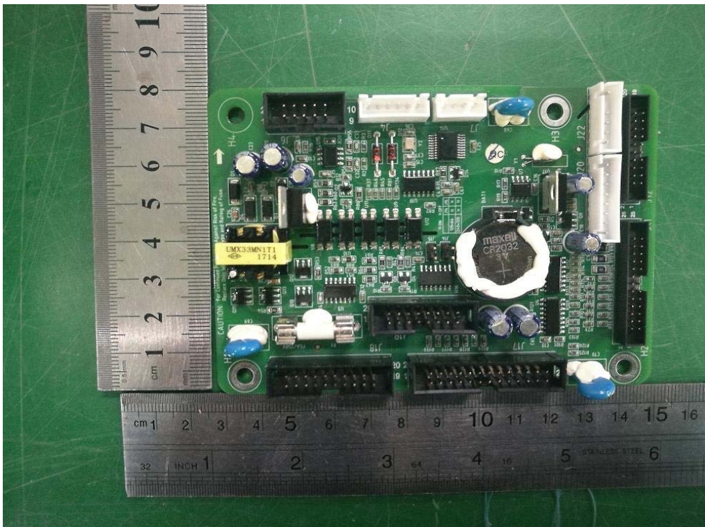
Figure 22: SELV PCB component view
