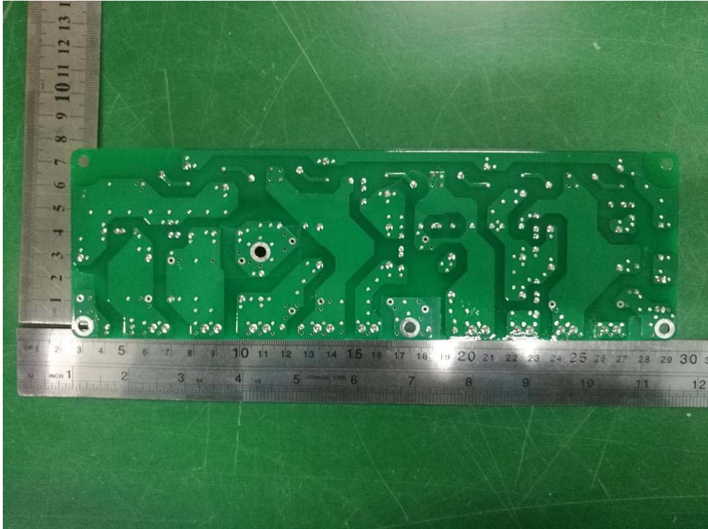
Figure 21: PCB trace view
