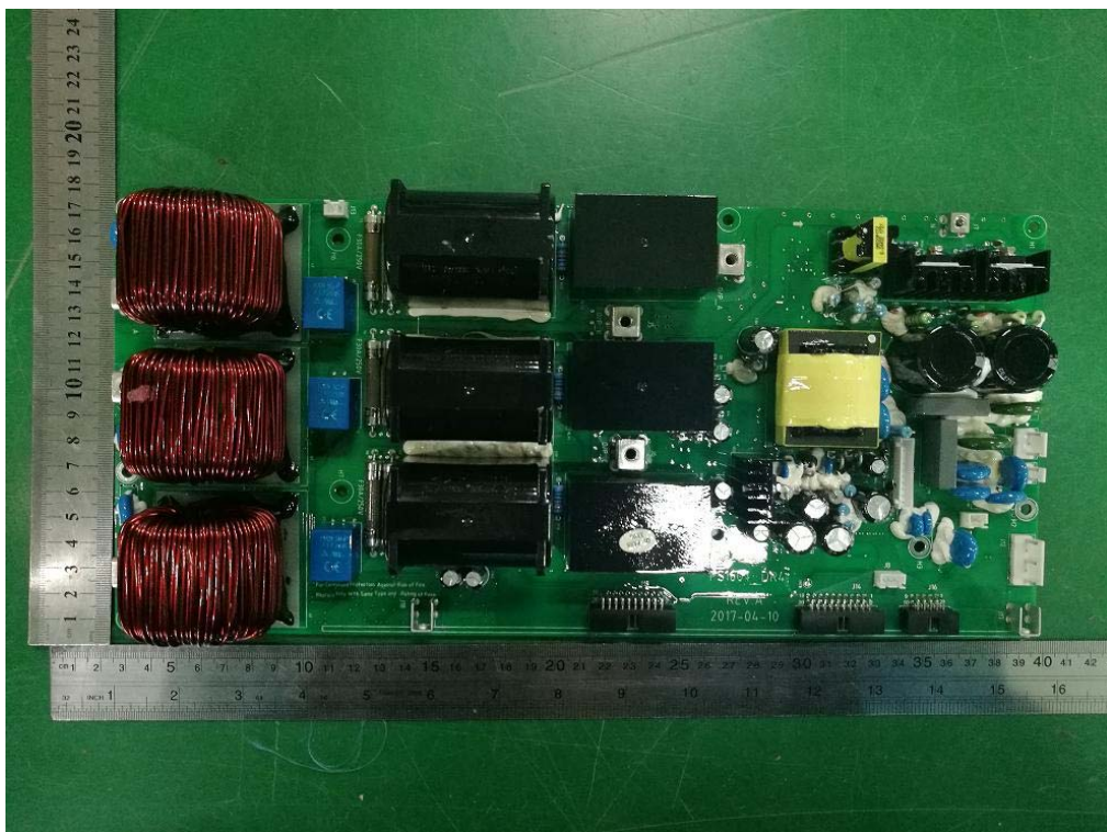
Figure 14: APS PCB component view
