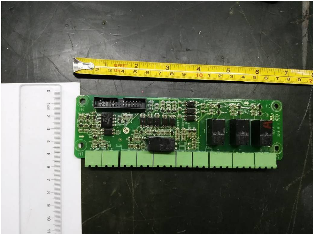
Fig. 18 –PCB view
