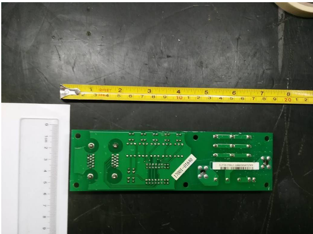
Fig. 21 – PCB view
