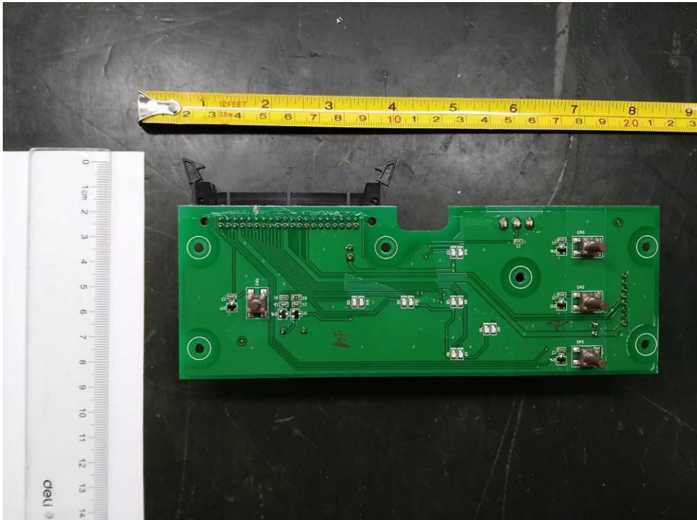
Fig. 10 – PCB view
