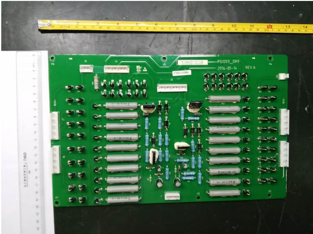
Fig. 8 –PCB view
