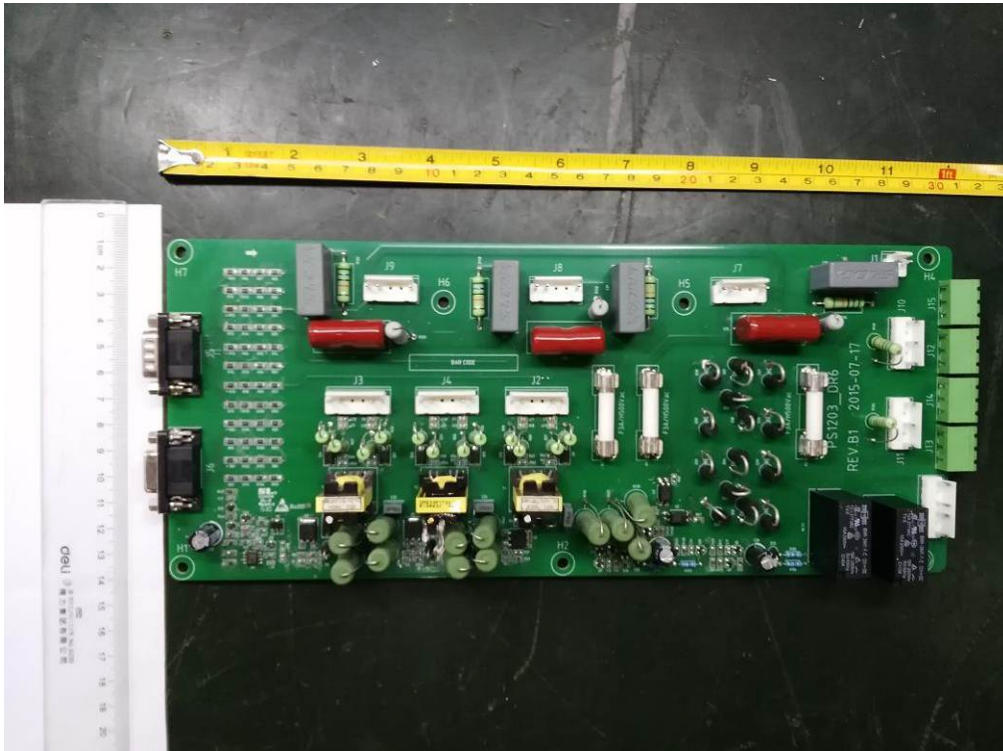
Fig. 6 – PCB view
