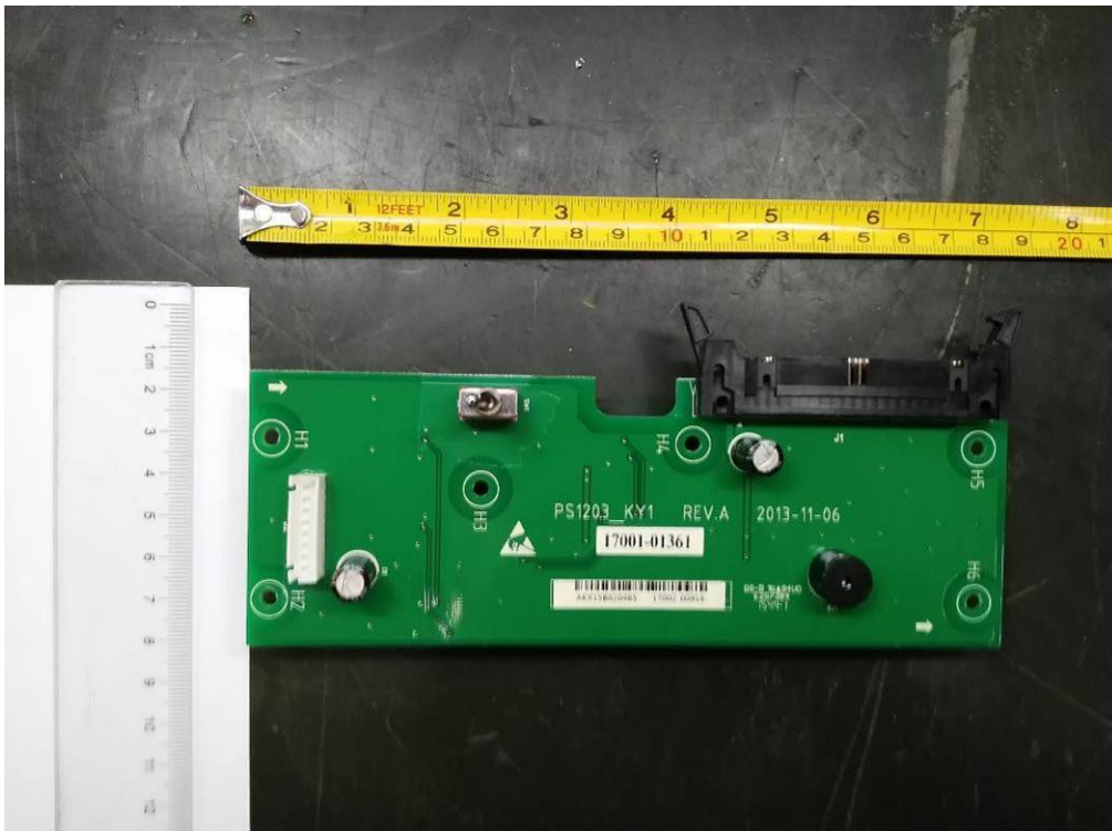
Fig. 11 – PCB view
