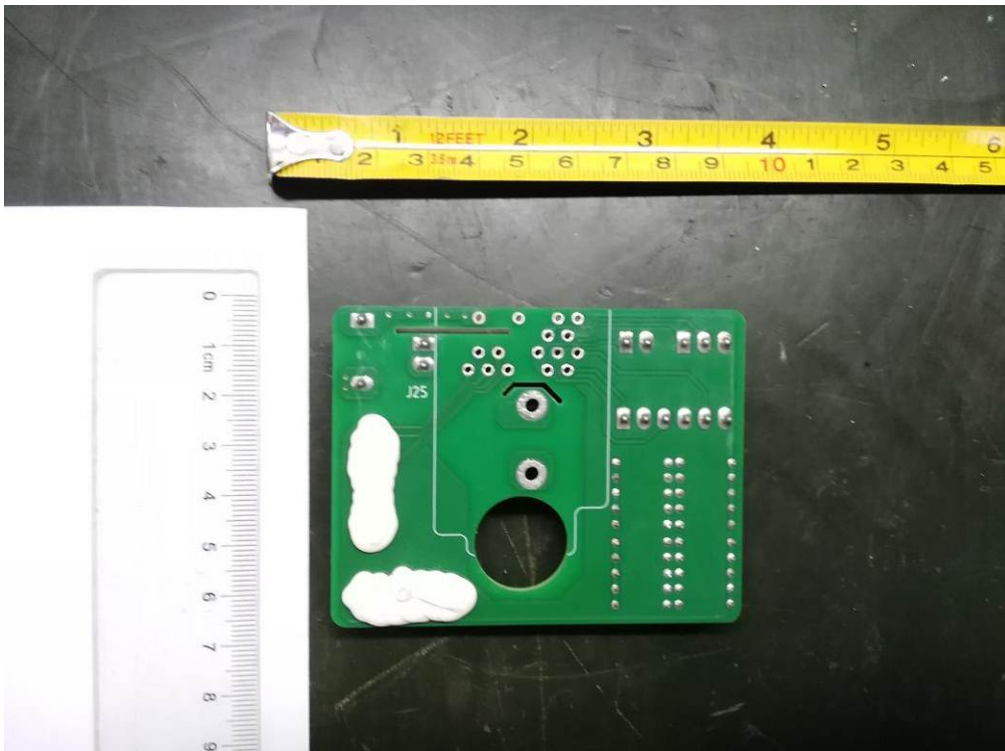
Fig. 17 – PCB view
