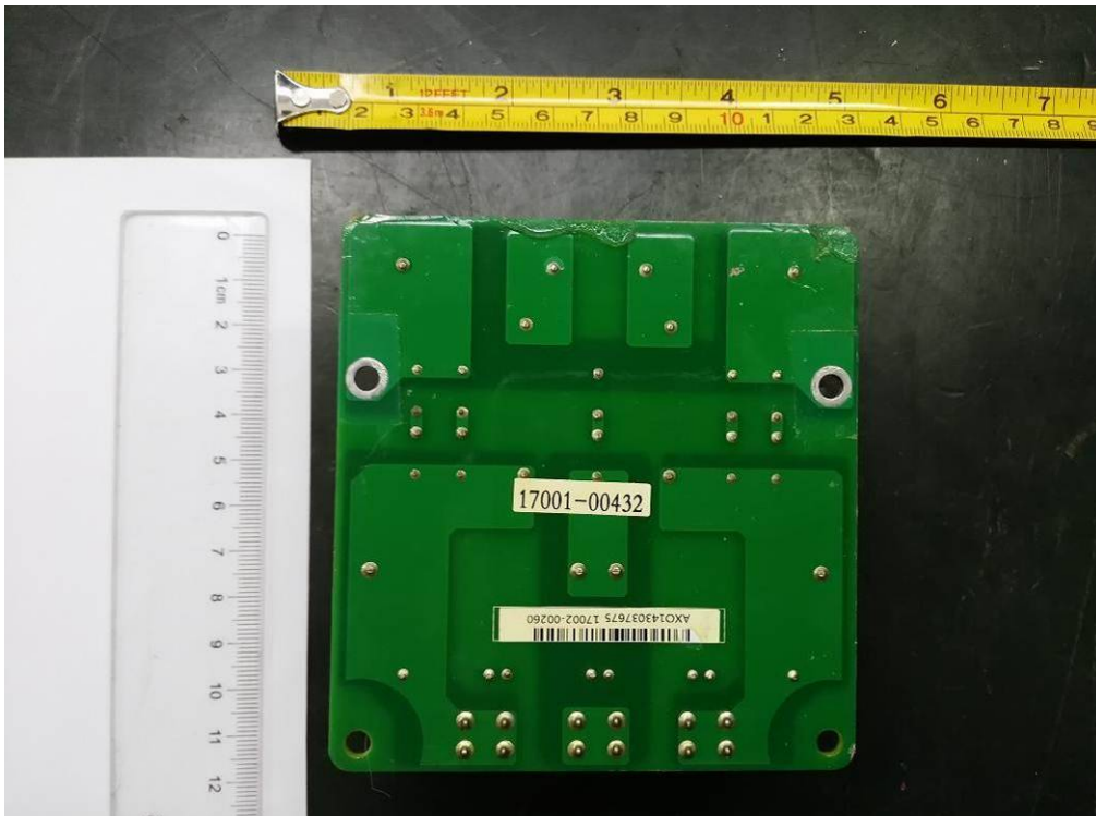
Fig. 5 – PCB view
