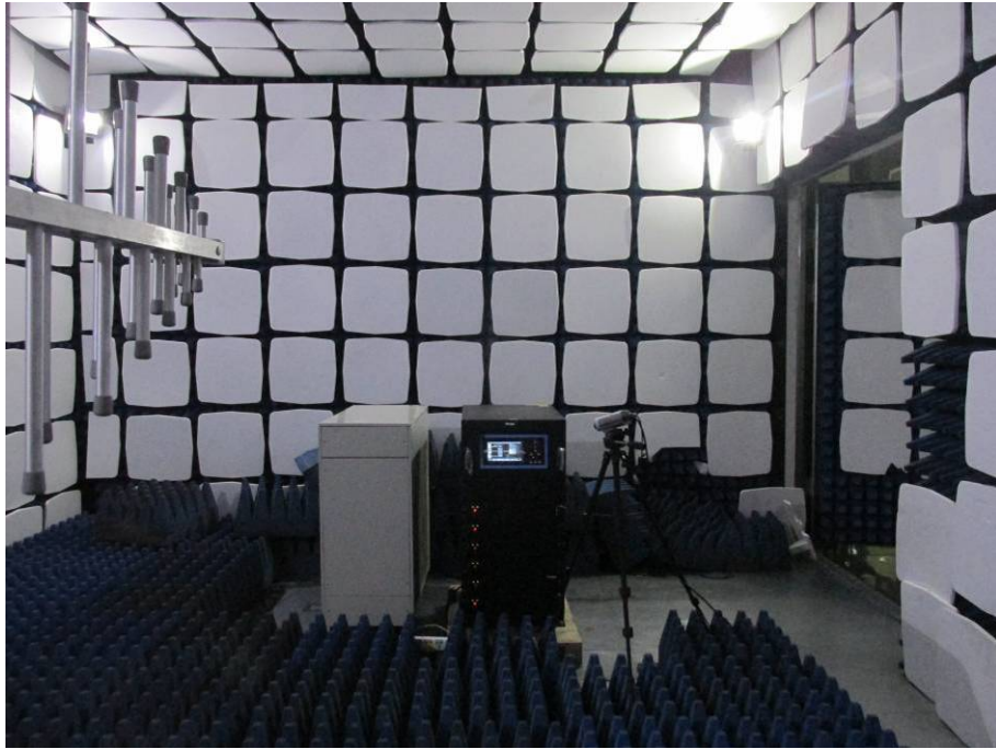
16.9.Photo of RF Field Strength Susceptibility Test
