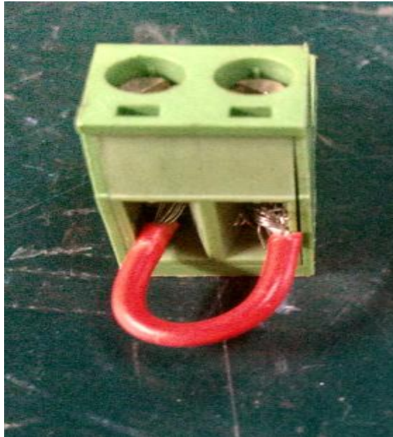
Figure 3 J4 terminal
