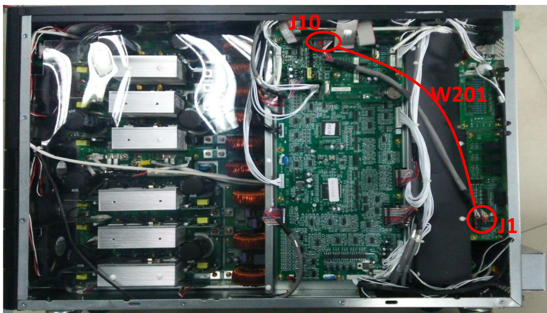
Figure 2 W201 cable
