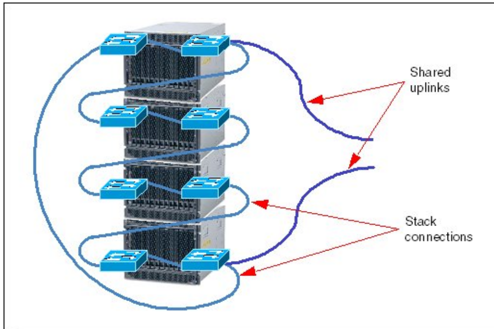
Figure 2. Virtual Blade Switch sample topology
