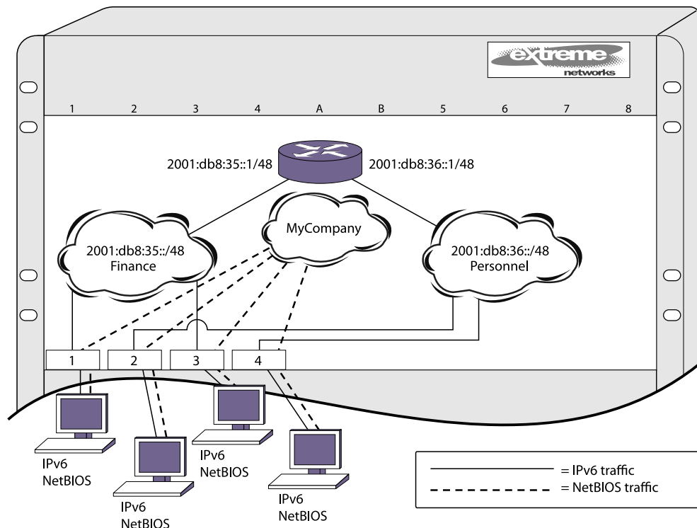
Figure 183: IPv6 Unicast Routing Configuration Example
