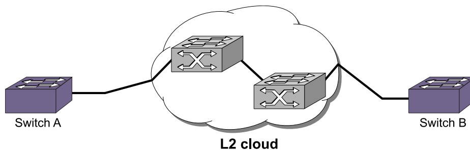
Figure 47: ELSM Through a Layer 2 Cloud
