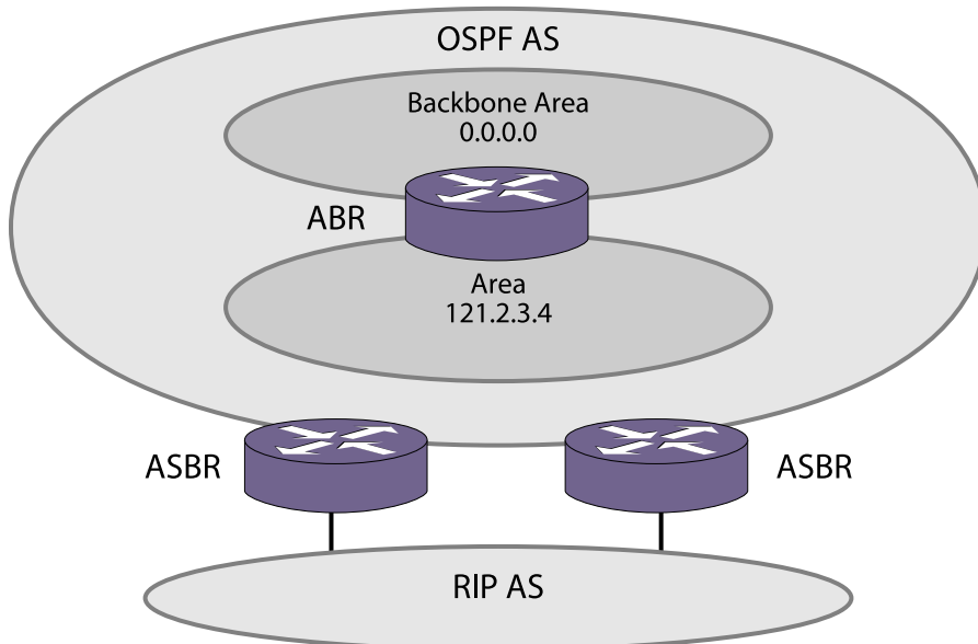
Figure 192: OSPF Route Redistribution
