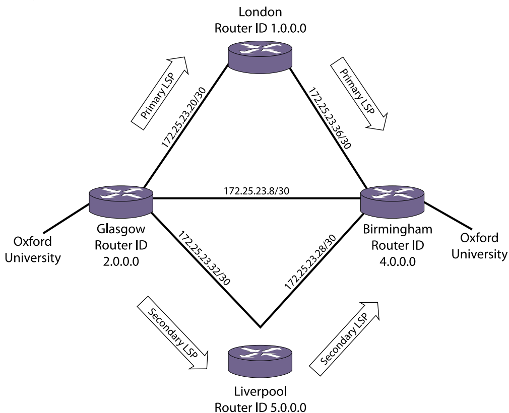
Figure 176: RSVP-TE Configuration Example
