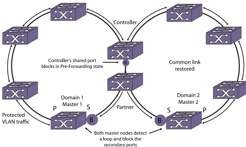
Figure 100: Common Link in Pre-Forwarding State
