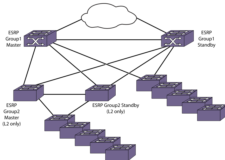
Figure 146: ESRP Groups
