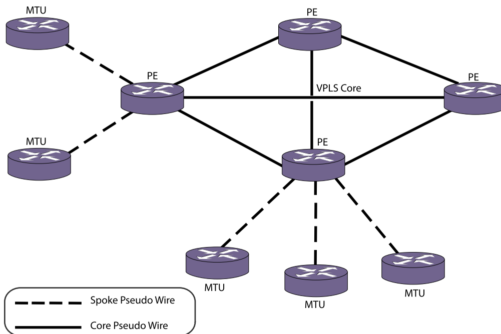
Figure 161: Example H-VPLS Network
