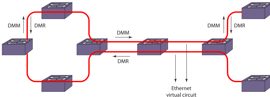
Figure 40: Two-Way Frame Delay and Frame Delay Variance Measurement
