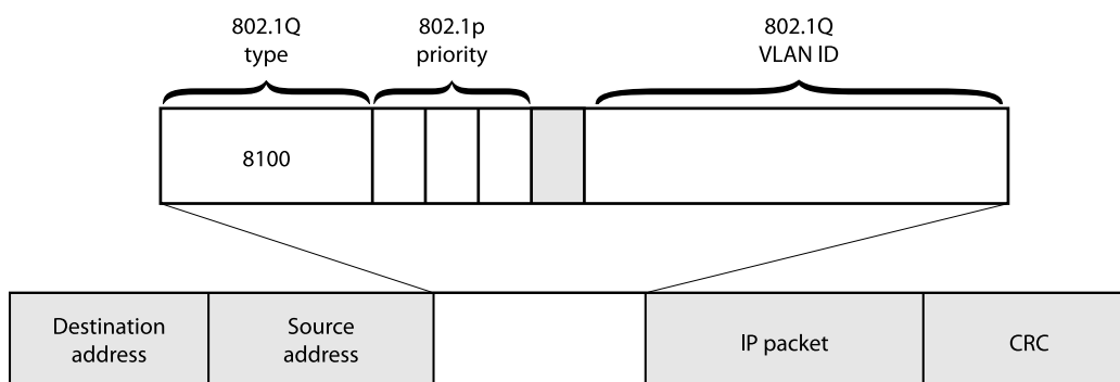
Figure 81: 802.1p Priority Bits
