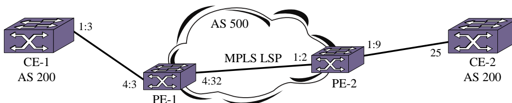
Figure 209: Layer 3 VPN
