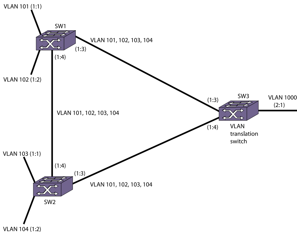
Figure 65: STP Redundancy Configuration Example
