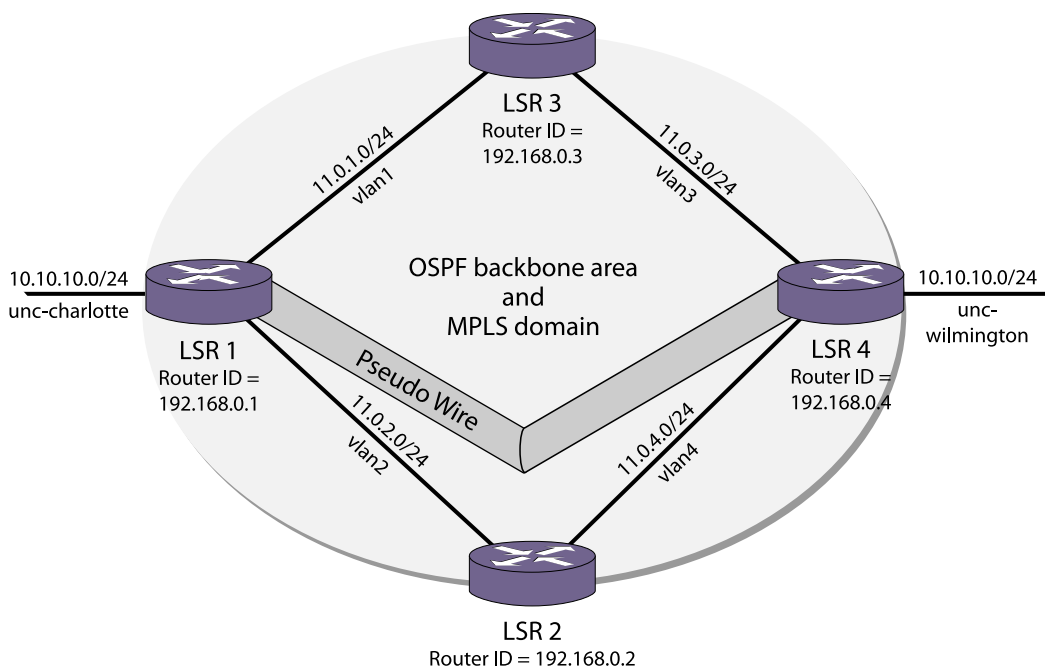
Figure 174: MPLS VPLS Configuration Example
