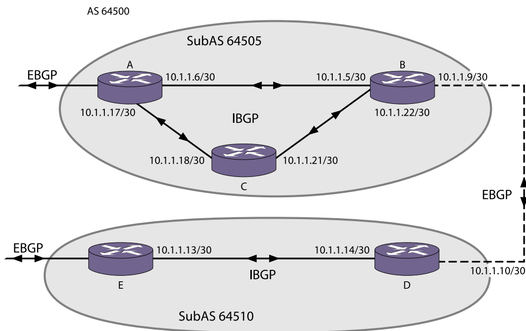
Figure 203: Routing Confederation
