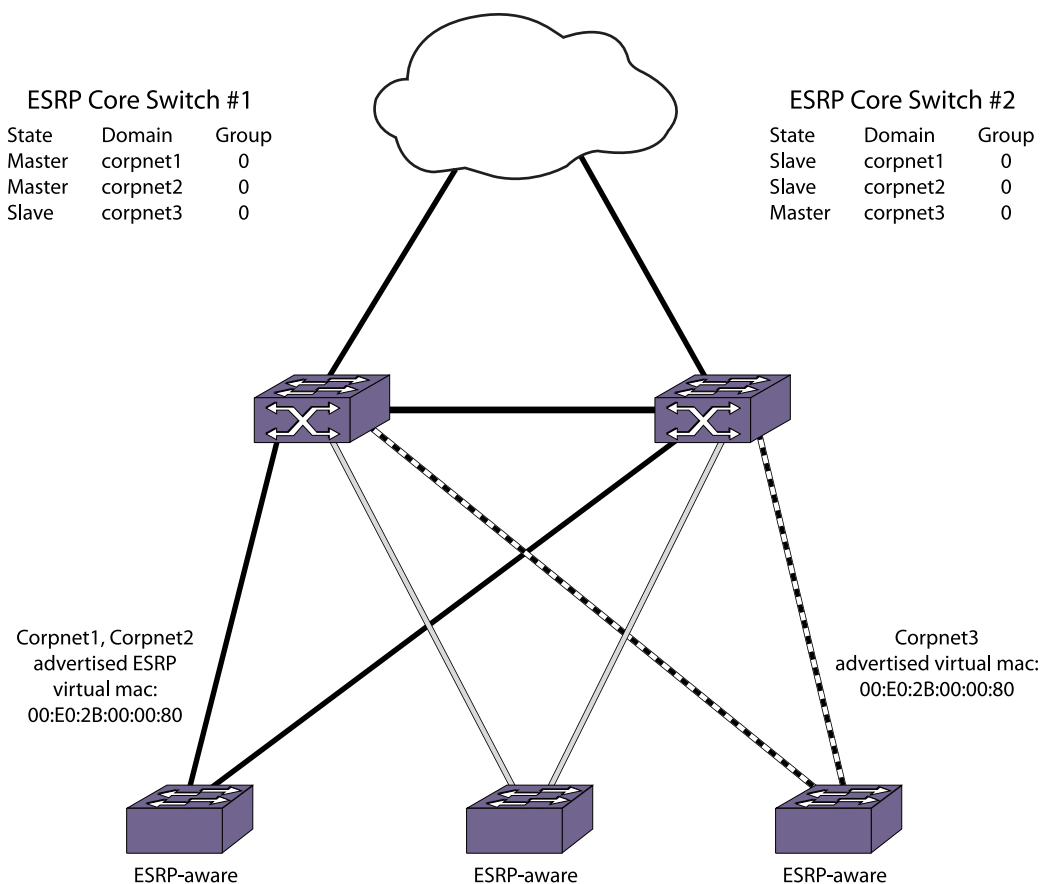
Figure 145: Example of a Basic ESRP Topology
