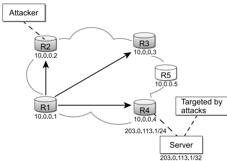
Figure 206: Black Hole Routing Using BGP
