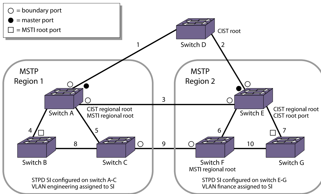
Figure 144: MSTP Configuration Example
