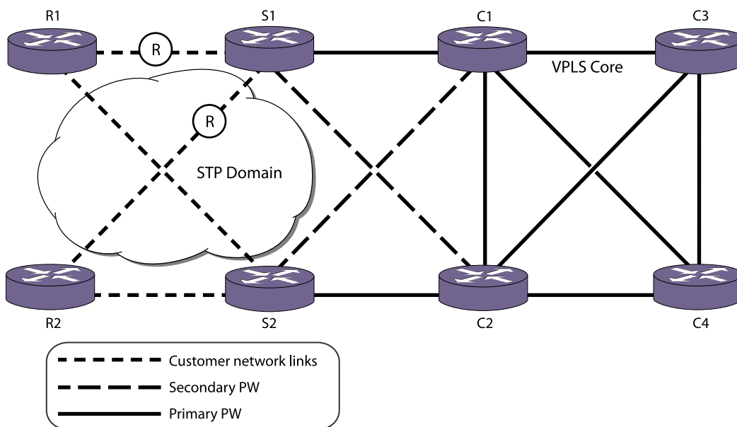
Figure 166: Redundant Edge H-VPLS Network with STP Example
