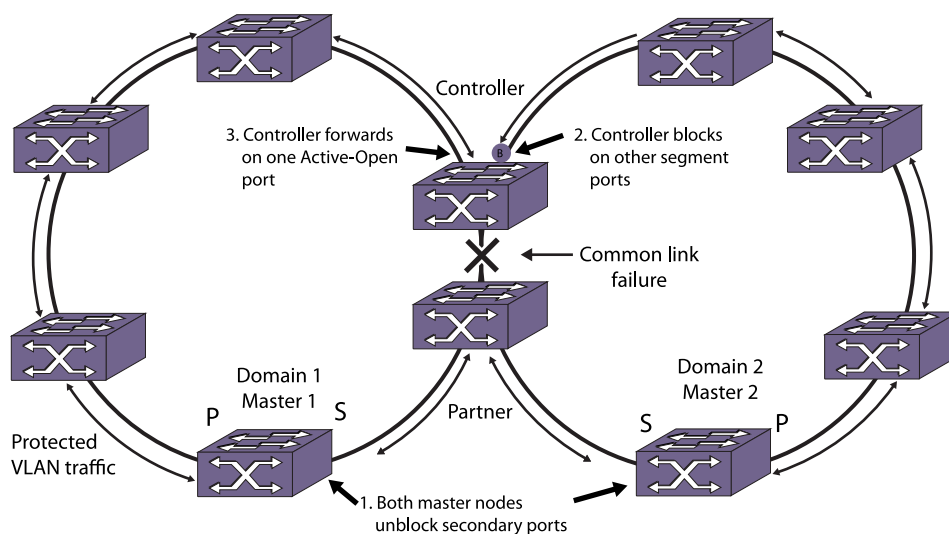
Figure 98: Common Link Failure
