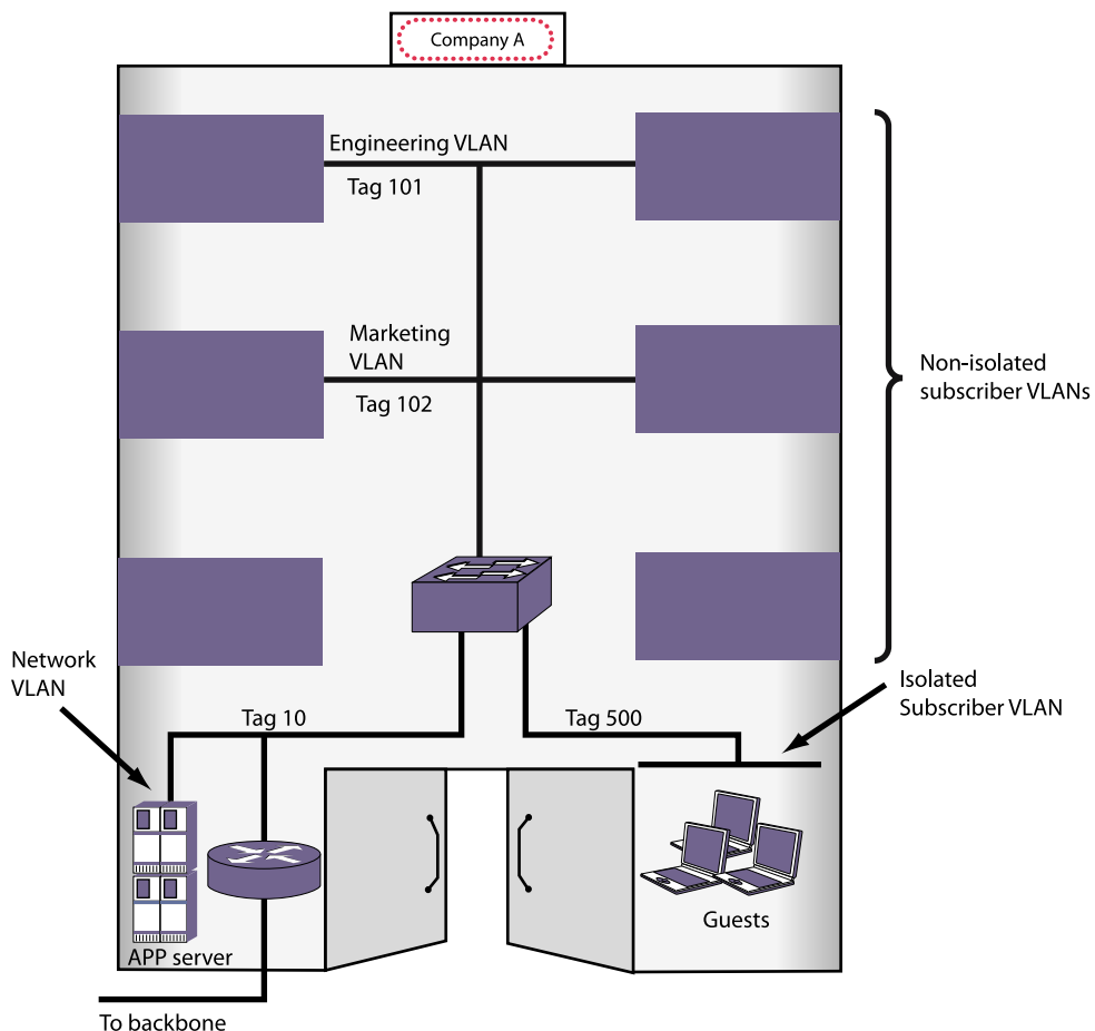
Figure 56: VLAN Isolation Application
