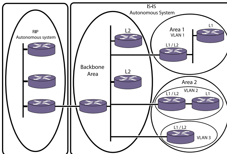
Figure 201: AS External Route Redistribution
