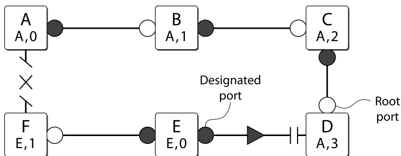
Figure 131: Communicating New Root Bridge Status to Neighbors
