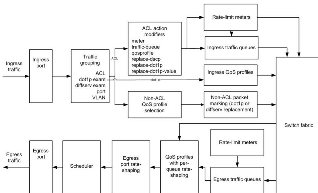
Figure 80: QoS on Extreme Networks Switches
