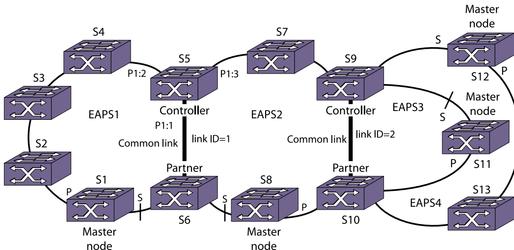
Figure 103: Basic Core Topology
