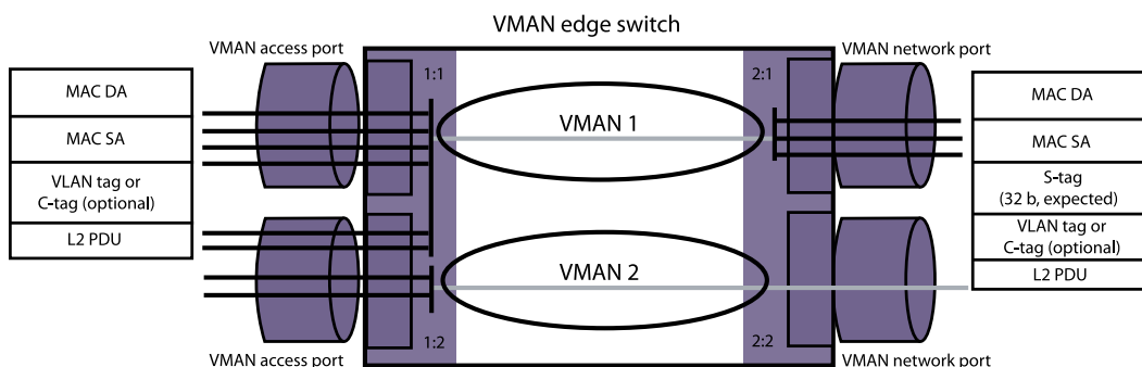
Figure 67: Tag Usage at the VMAN Access Switch
