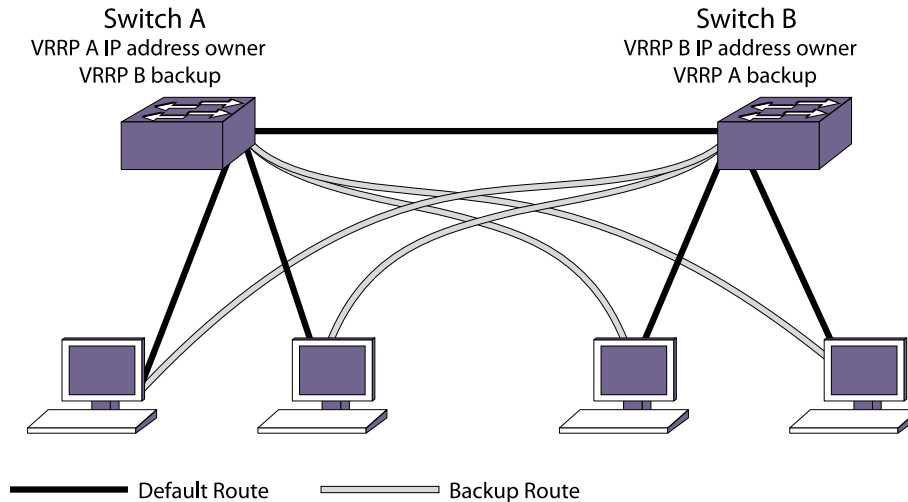
Figure 152: VRRP Load-Sharing Configuration
