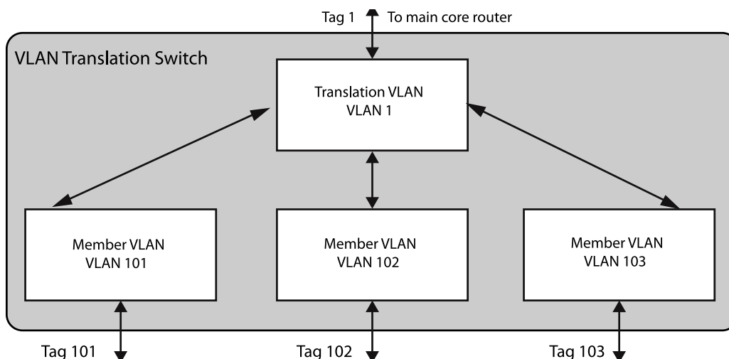
Figure 62: VLAN Translation Switch Configuration
