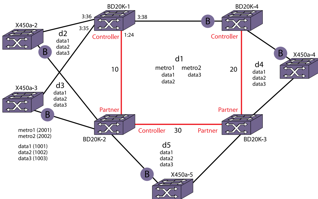
Figure 115: Sample EAPS Topology with PBB
