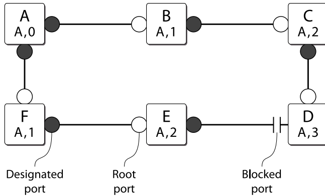
Figure 128: Initial Network Configuration
