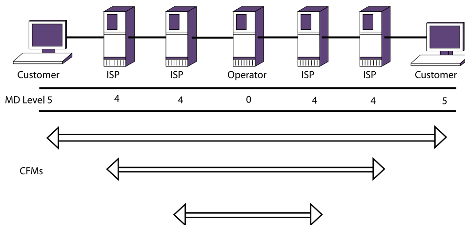
Figure 37: CFM Hierarchical Domains Example
