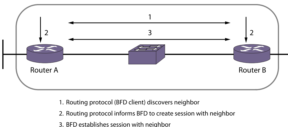
Figure 45: BFD Topology
