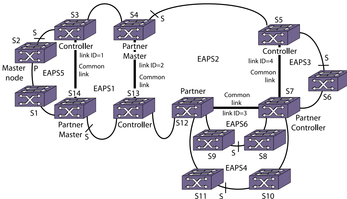
Figure 106: Advanced Basic Core and Right Angle Topology
