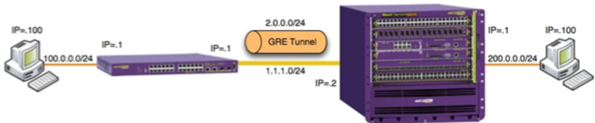
Figure 178: GRE Tunnel Configuration
