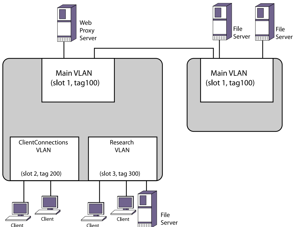
Figure 60: PVLAN Configuration Example 1
