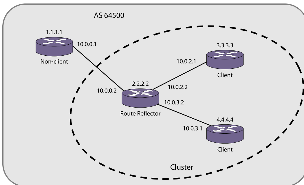
Figure 202: Route Reflectors
