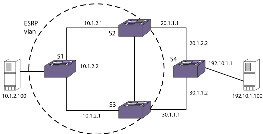
Figure 88: MAC Address Limits and VLANs Participating in ESRP
