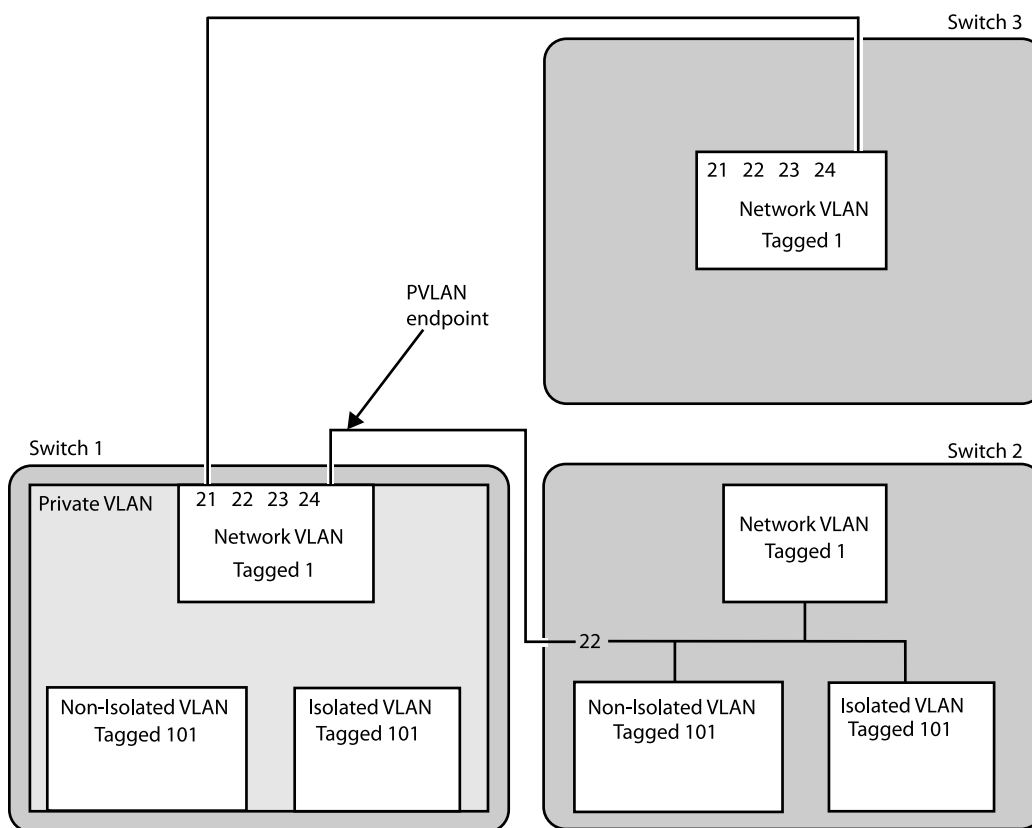
Figure 59: Private VLAN Connections to Switches Outside the PVLAN
