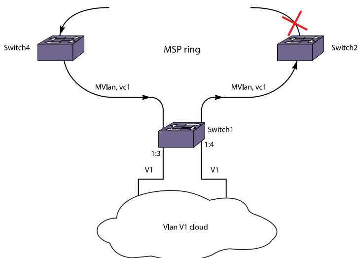
Figure 224: MVR with STP
