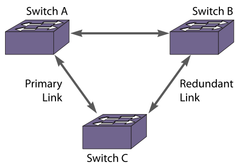
Figure 35: Dual-Homed Implementation for Switch C
