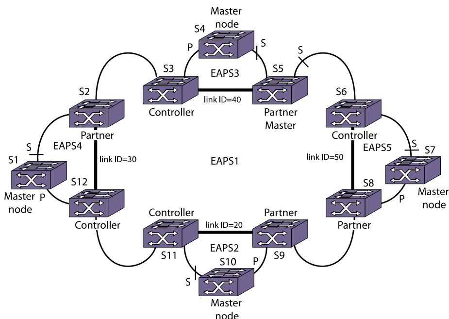
Figure 107: Large Core and Access Ring Topology
