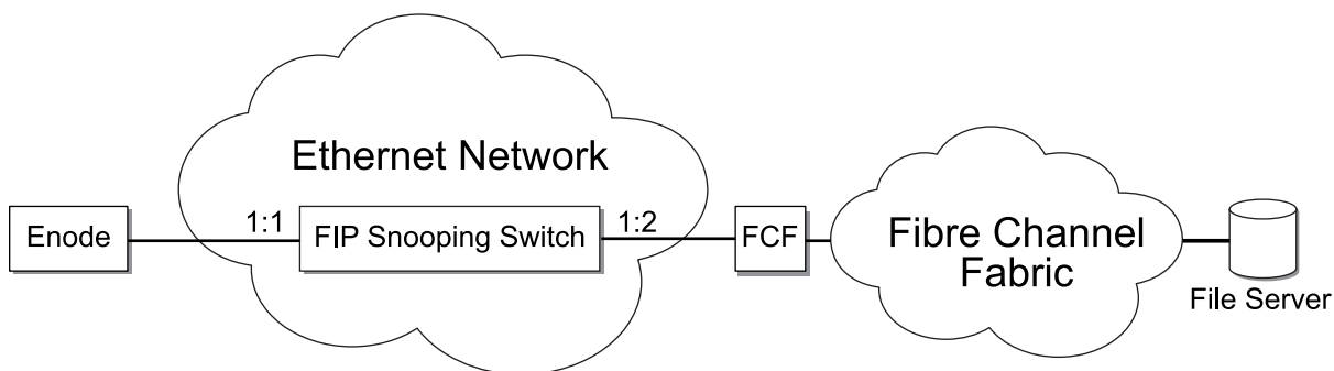
Figure 75: Example FIP Snooping Configuration
