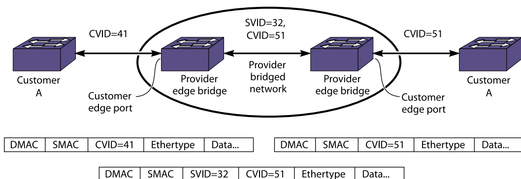
Figure 69: CVID Translation
