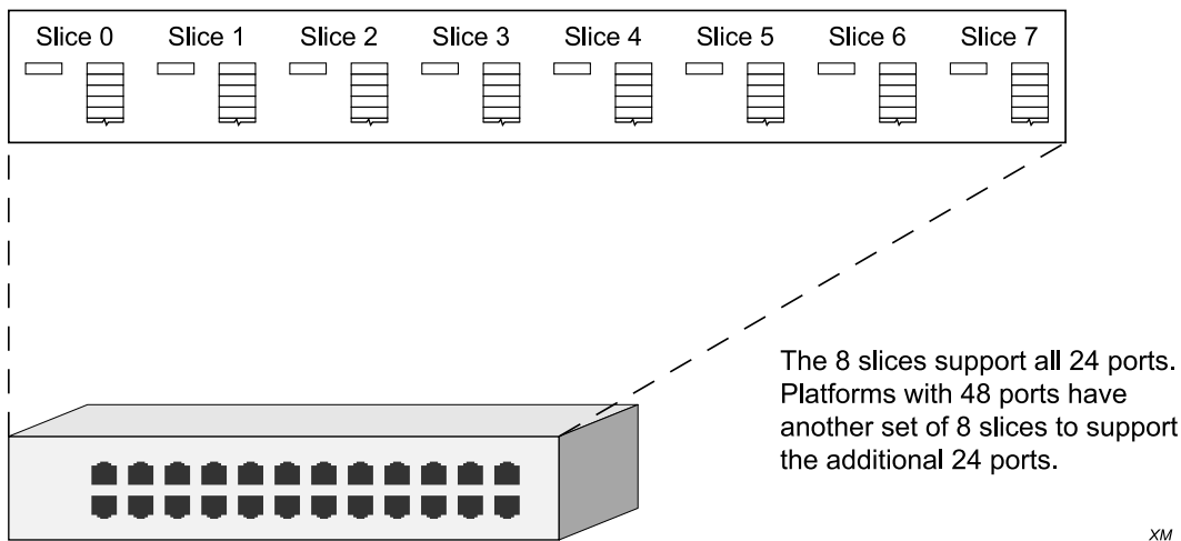
Figure 77: Slice Support for Summit X150, X250e, X350, and X450e Series Switches and BlackDiamond 8000 e-Series Modules
