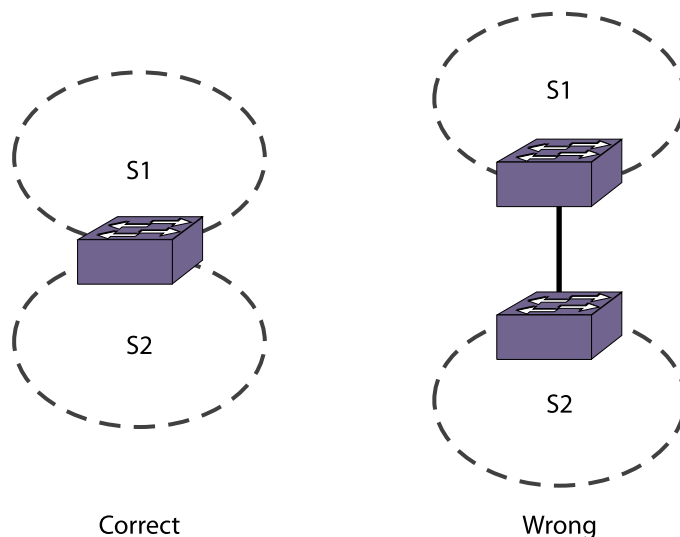
Figure 125: VLANs Traverse Domains Inside Switches
