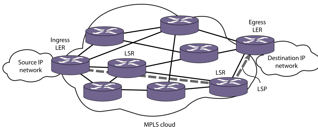
Figure 155: MPLS Network
