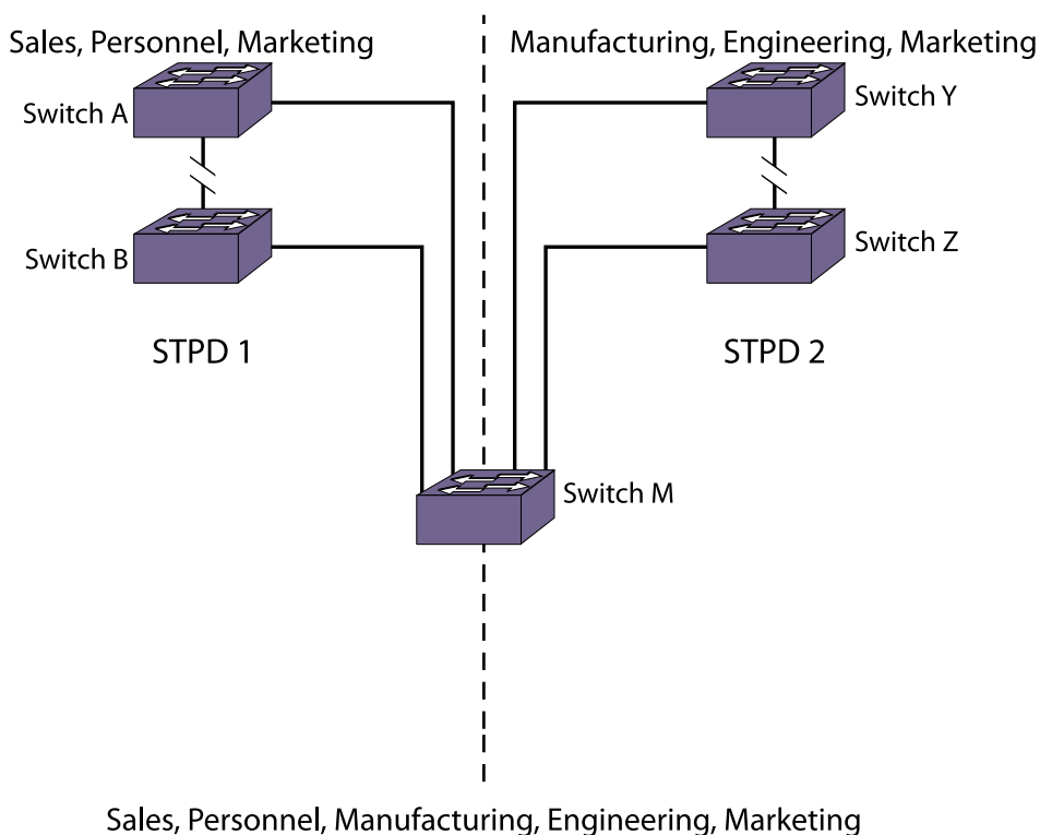
Figure 143: RSTP Example
