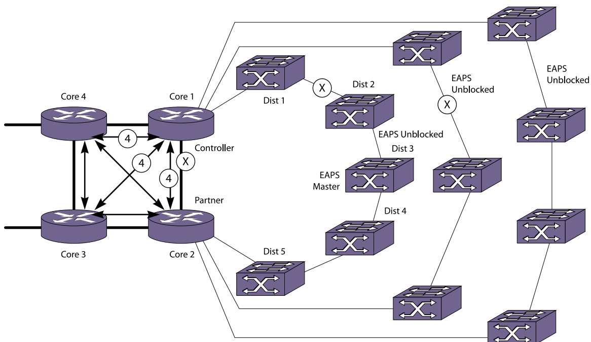
Figure 168: VPLS with Parallel Redundant EAPS Rings Configuration Example
