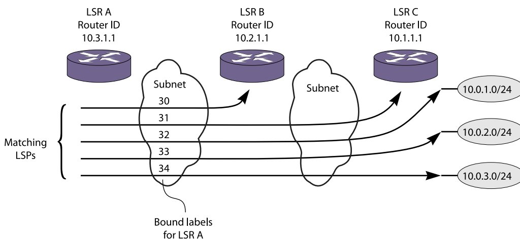
Figure 160: Matching and Calculated LSP Next Hops
