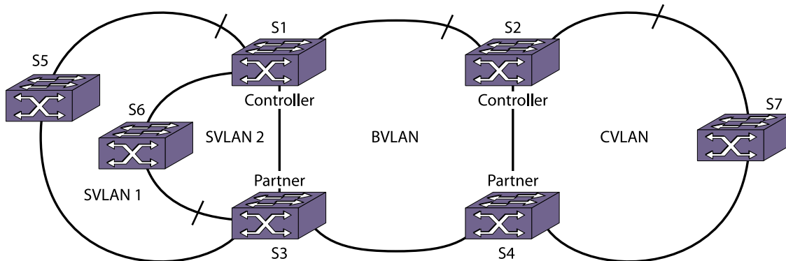
Figure 99: Combined EAPS and PBBN Topology
