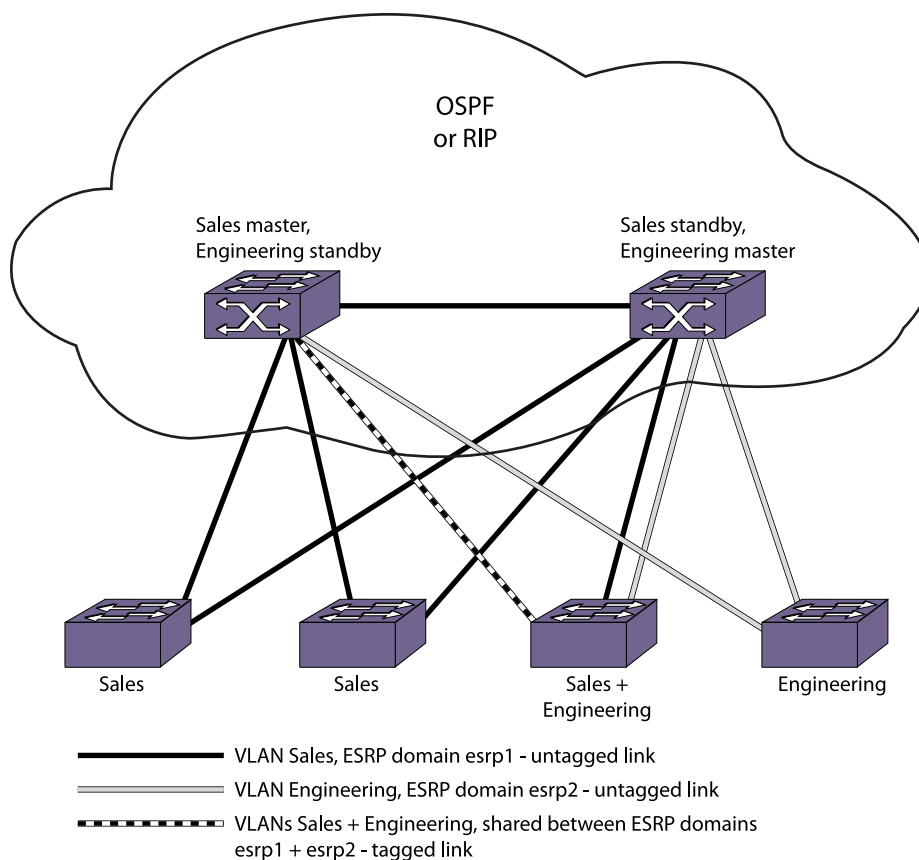
Figure 150: Multiple ESRP Domains Using Layer 2 and Layer 3 Redundancy
