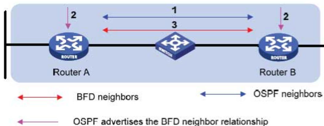
Figure 188: Basic Operational Flow of OSPF BFD
