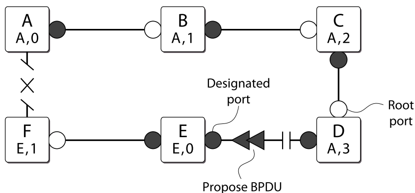
Figure 132: Sending a Propose Message to Confirm a Port Role
