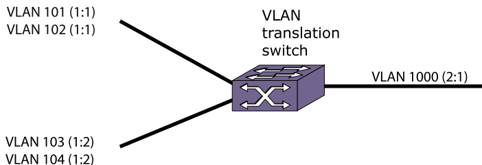
Figure 63: VLAN Translation Configuration Example
