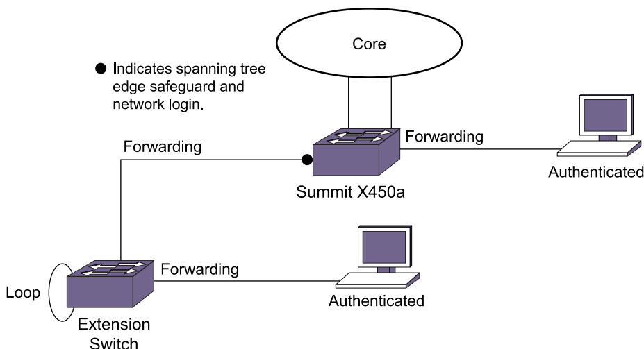
Figure 141: Traffic Monitoring on the Edge Side
