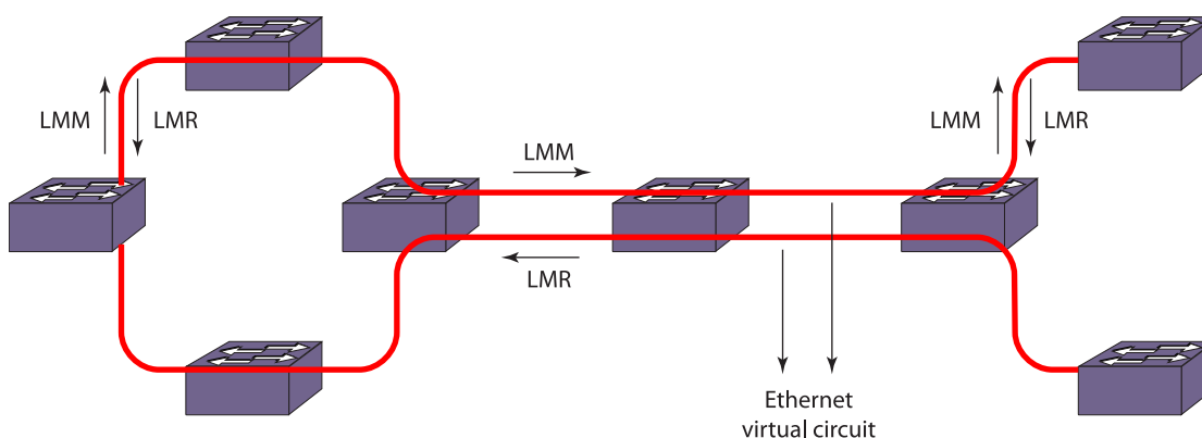
Figure 42: Two-Way Frame-Loss Measurement
