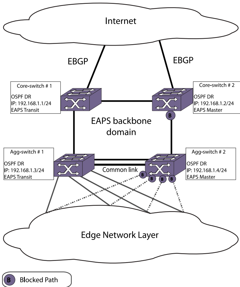
Figure 113: Core EAPS and OSPF Network Layer
