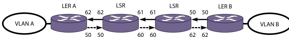
Figure 171: Static LSP Example
