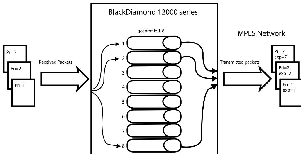
Figure 172: Mapping Dot1p to EXP Bits
