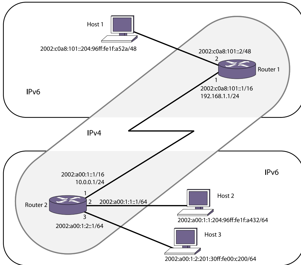
Figure 185: 6to4 Tunnel Configuration Example
