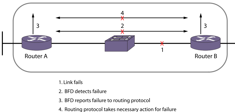
Figure 46: BFD Failure Detection
