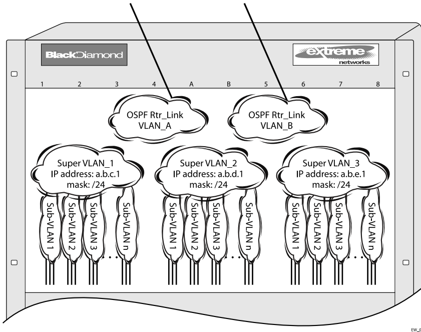
Figure 182: VLAN Aggregation
