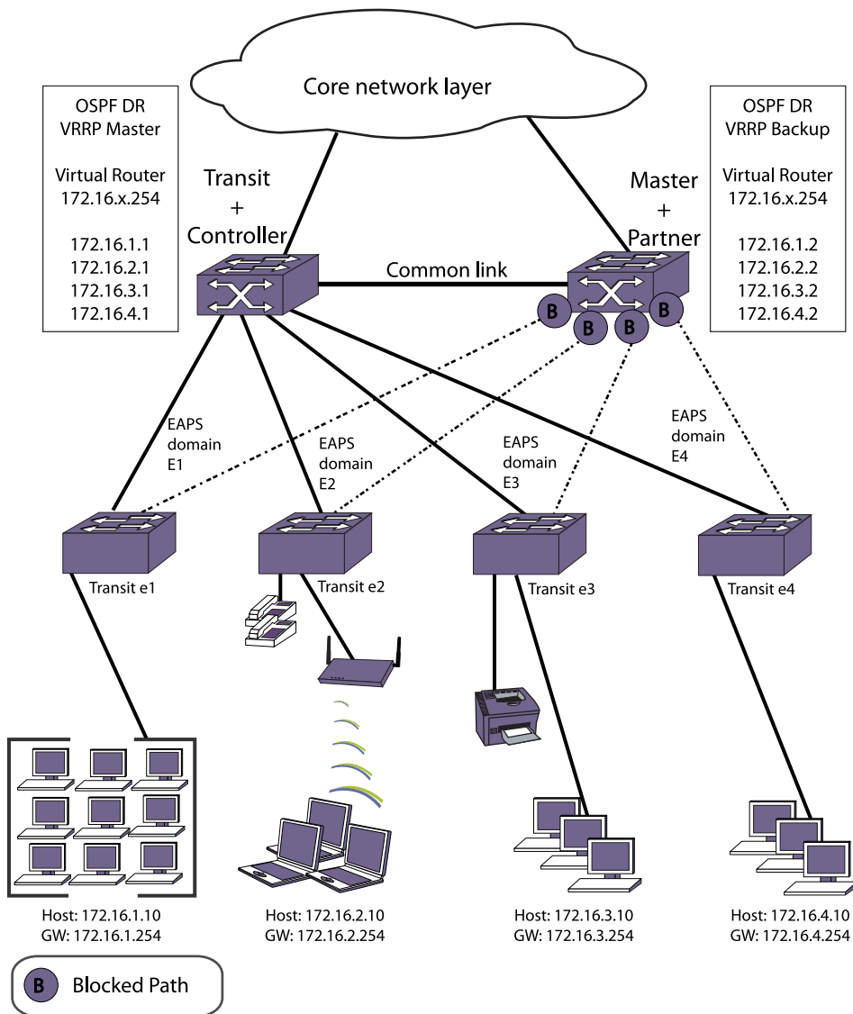
Figure 112: L2 and L3 Aggregation Network Layer
