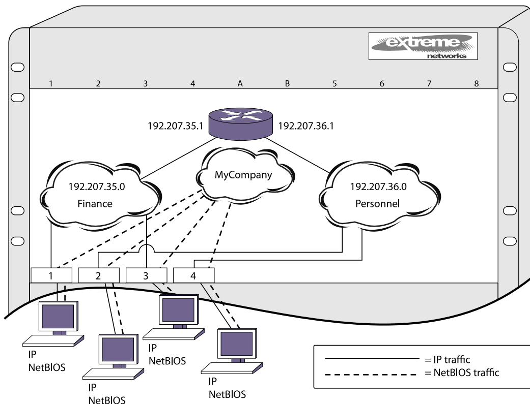
Figure 180: Unicast Routing Configuration Example
