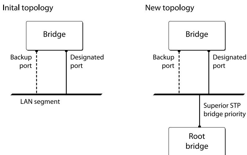
Figure 127: Example of Root Port Rapid Behavior
