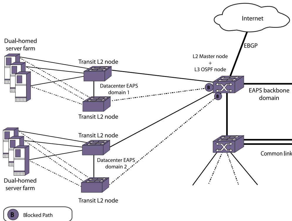
Figure 114: Datacenter EAPS and OSPF Network Layer
