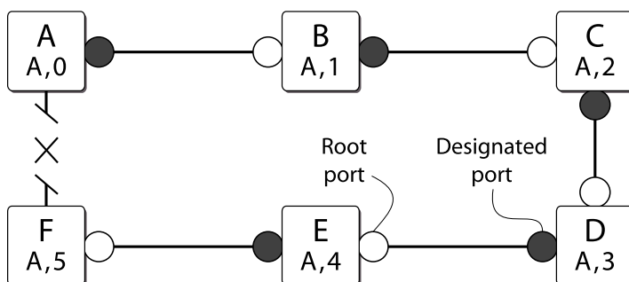
Figure 135: Final Network Configuration
