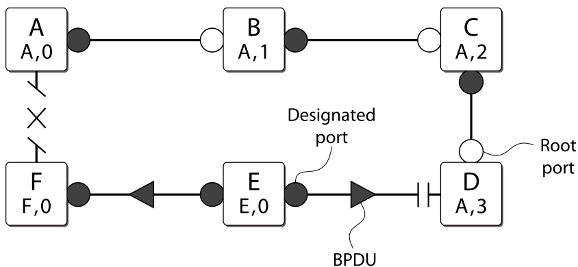
Figure 130: New Root Bridge Selected
