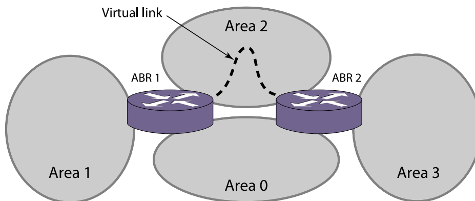
Figure 191: Virtual Link Providing Redundancy
