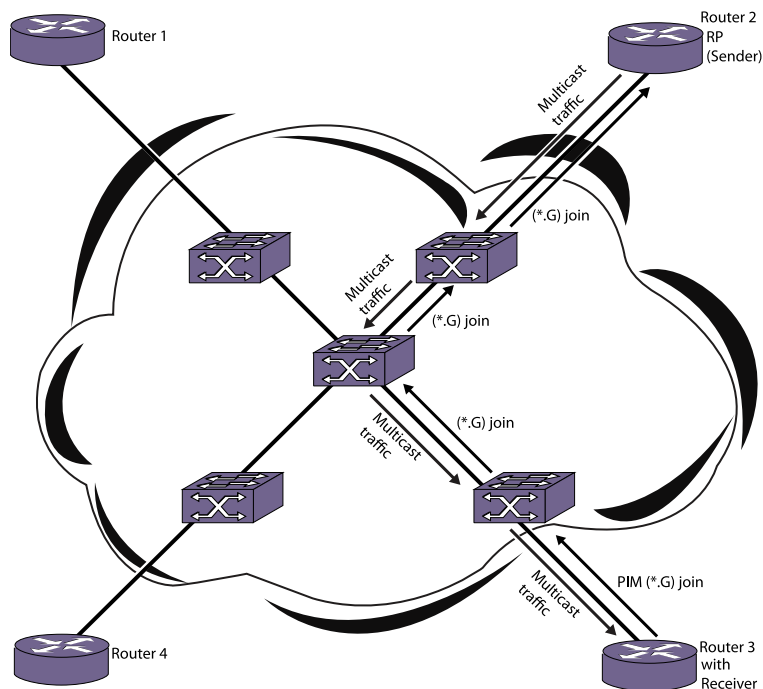
Figure 215: Multicast With PIM Snooping
