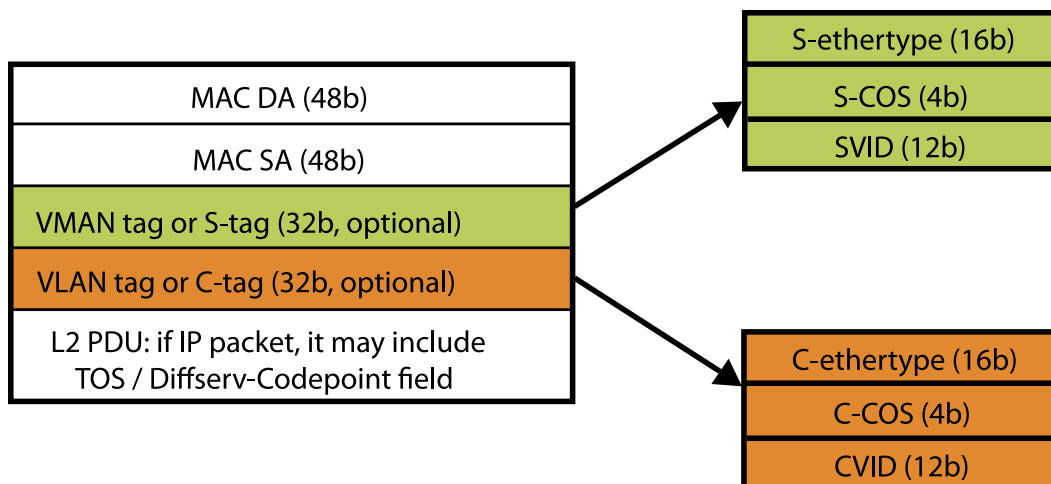
Figure 68: S-tag and C-tag Components
