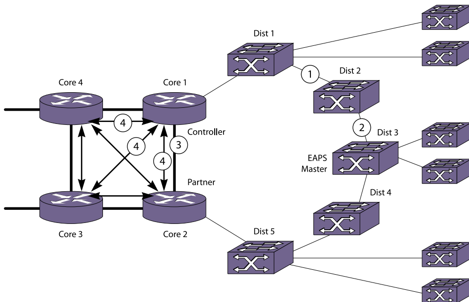
Figure 167: VPLS with Redundant EAPS Configuration Example
