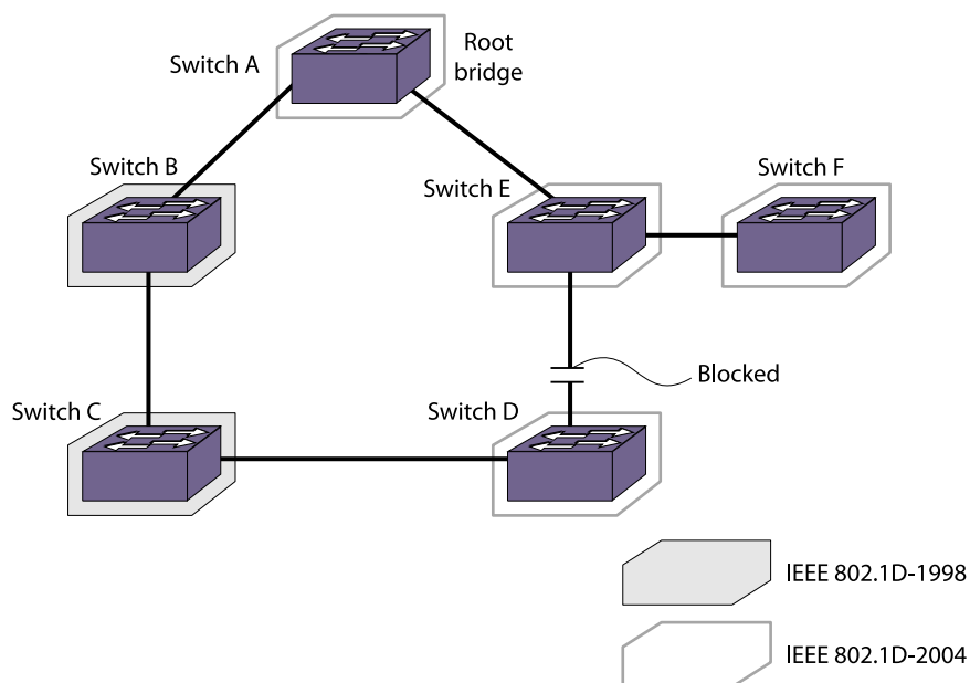
Figure 118: 802.1D-1998 and 802.1D-2004 Mixed Bridge Topology
