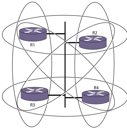
Figure 198: Point-to-Point Adjacencies in a Four-Router Network
