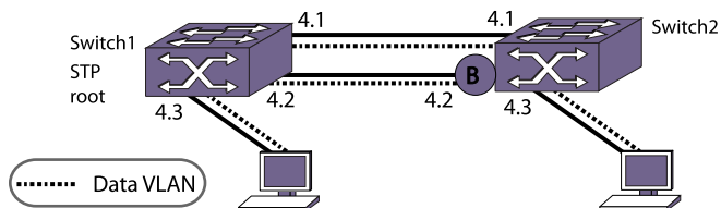
Figure 108: Sample STP Network for Migration to EAPS
