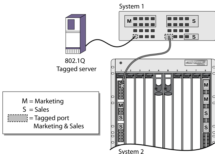
Figure 52: Physical Diagram of Tagged and Untagged Traffic
