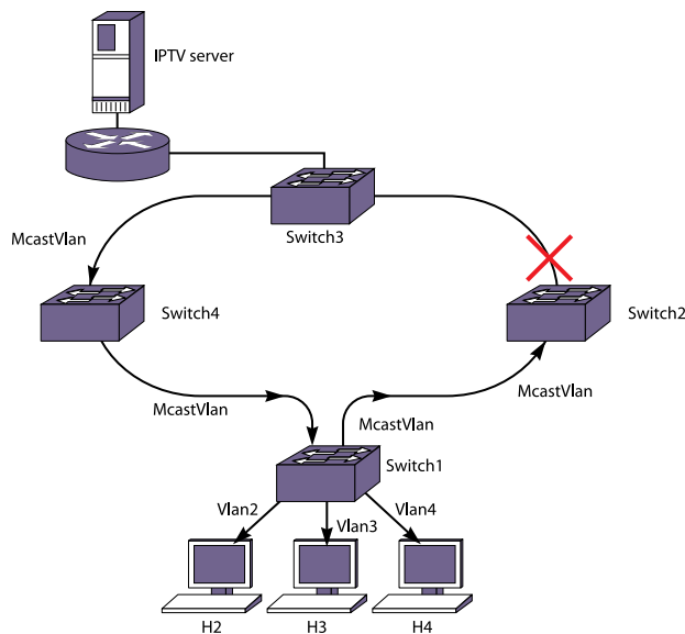
Figure 220: Basic MVR Deployment
