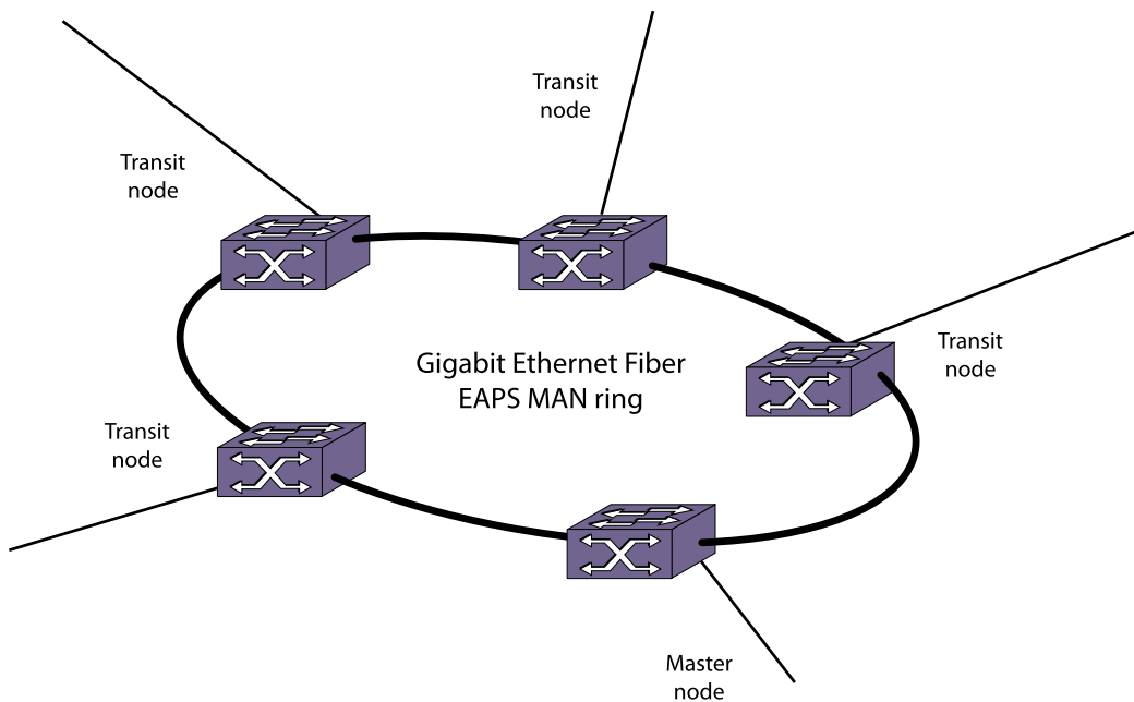
Figure 93: Gigabit Ethernet Fiber EAPS MAN Ring
