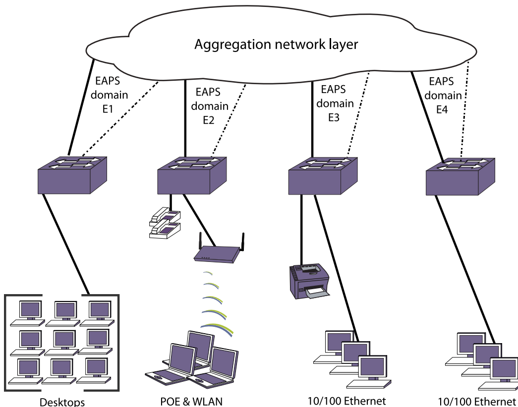
Figure 110: Converged Network Edge (Unified Access Layer)
