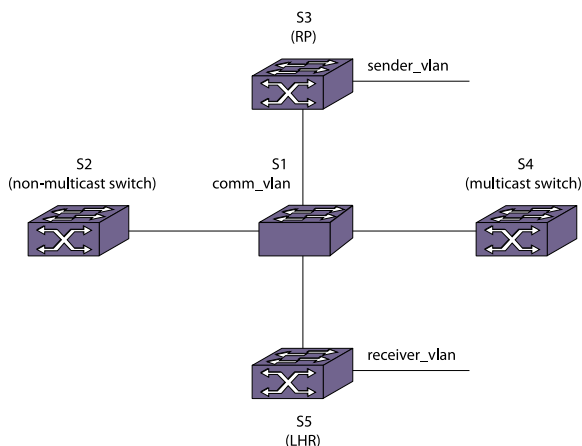
Figure 218: PIM Snooping Configuration Example
