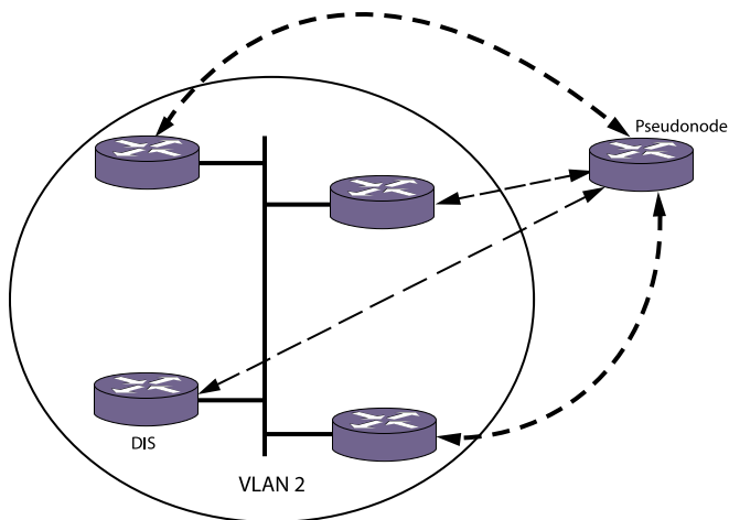
Figure 199: Broadcast Adjacencies in a Four-Router Network
