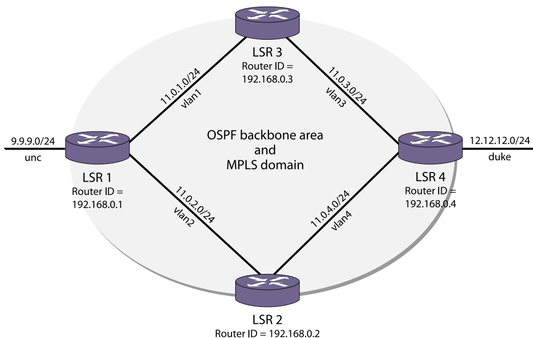
Figure 173: MPLS Configuration Example
