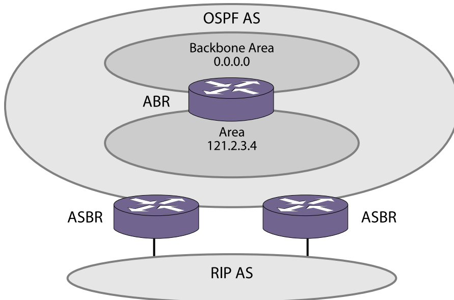
Figure 196: Route Redistribution
