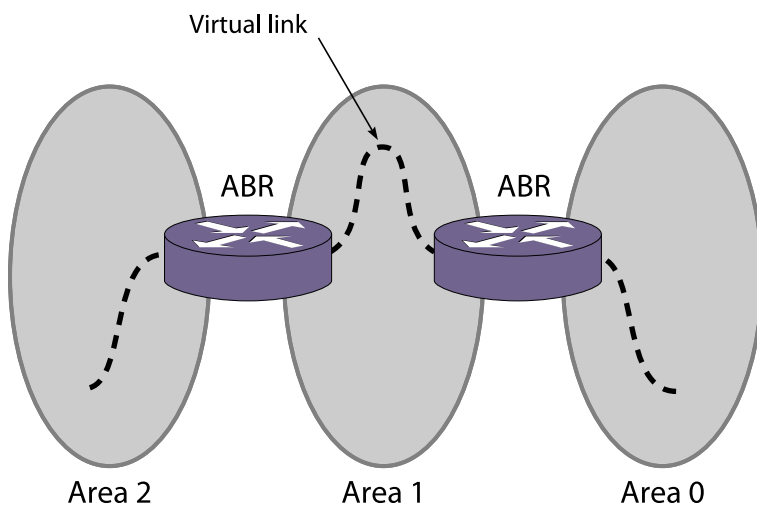
Figure 194: Virtual Link Using Area 1 as a Transit Area
