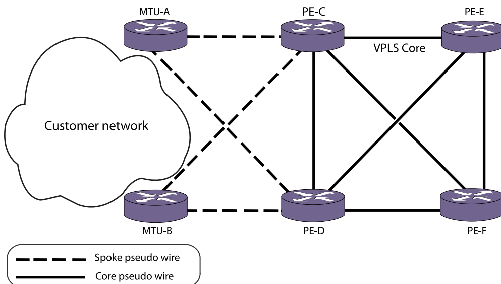
Figure 165: Example Redundant Edge H-VPLS Network
