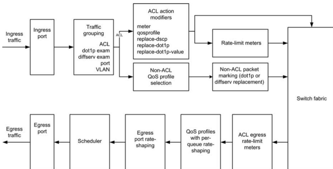
Figure 83: QoS on BlackDiamond X8 and 8800 Series Switches, SummitStack, and Summit Family Switches
