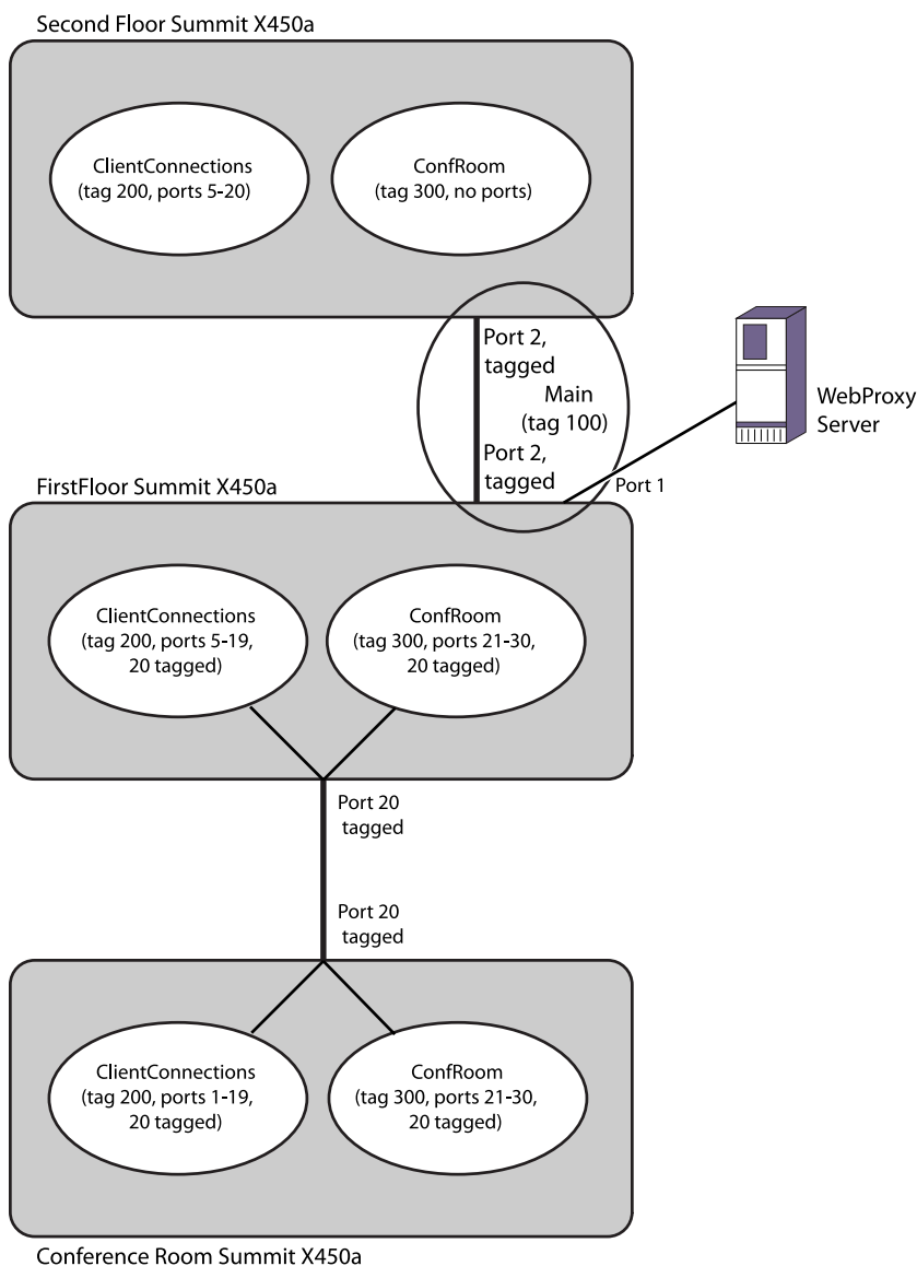
Figure 61: PVLAN Configuration Example 2
