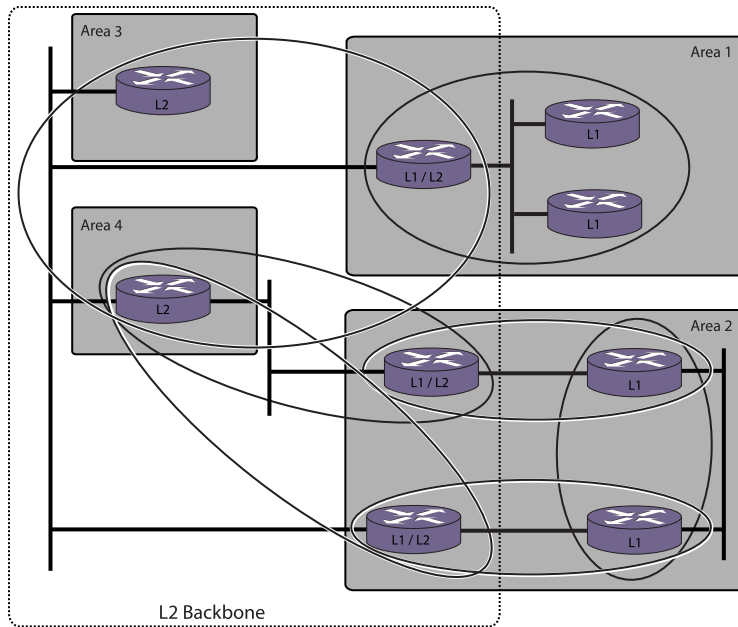
Figure 200: Basic Autonomous System
