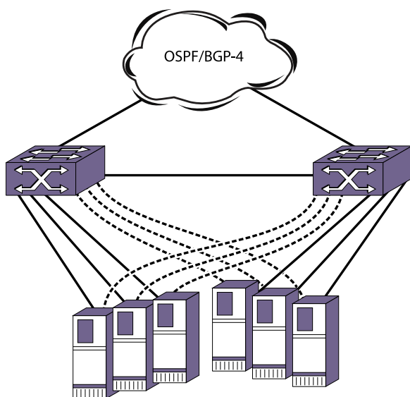
Figure 148: ESRP Host Attach
