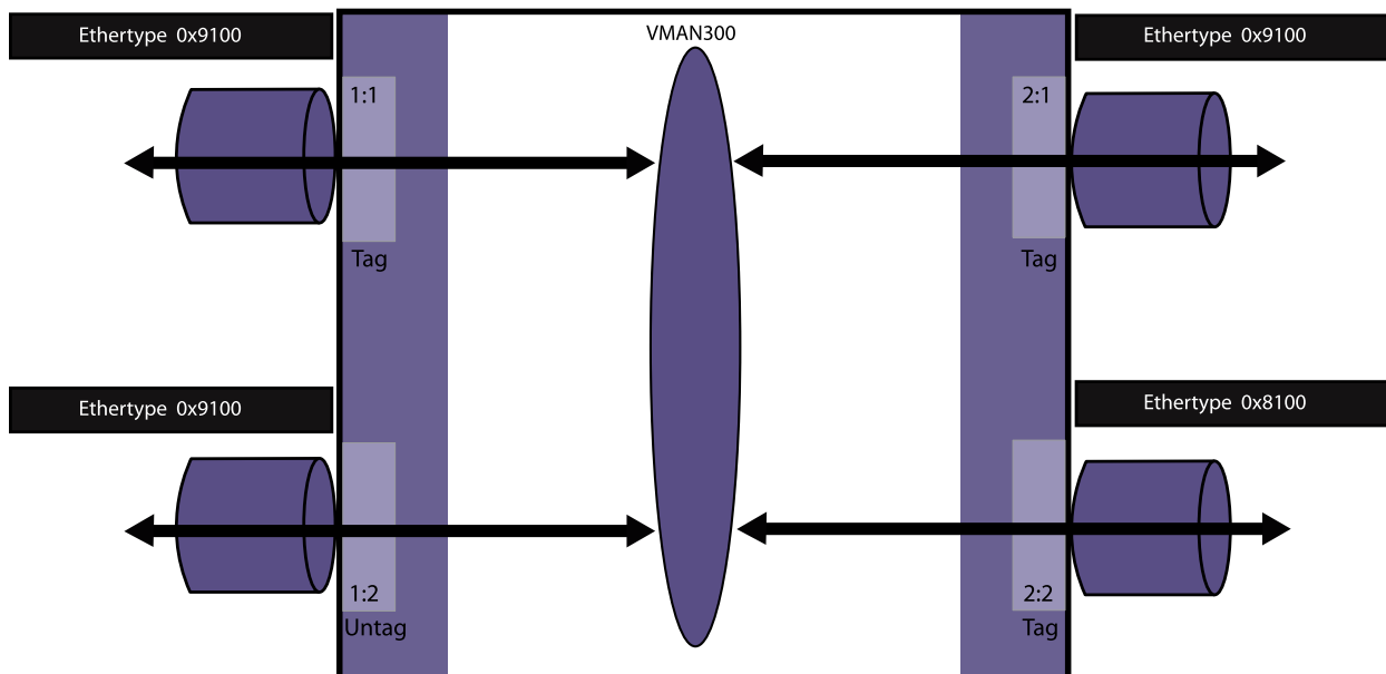
Figure 72: Multiple VMAN Ethertype Example
