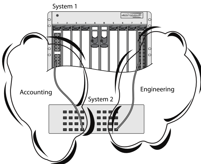
Figure 51: Two Port-based VLANs Spanning Two Switches
