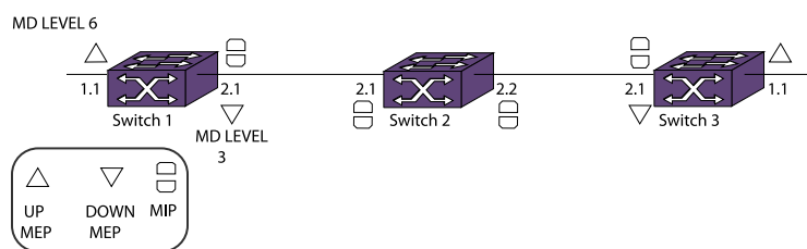
Figure 39: CFM Configuration Example
