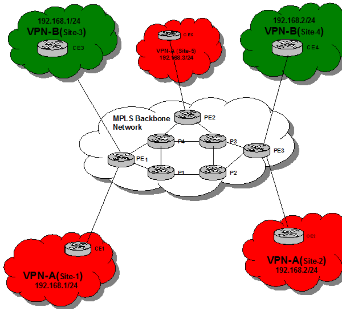
Figure 211: BGP/MPLS VPN Example
