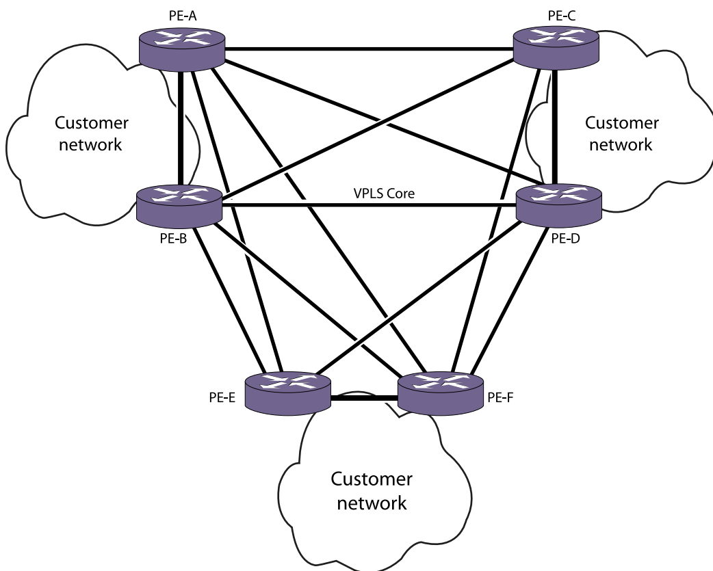
Figure 163: Example Protected Access VPLS Network
