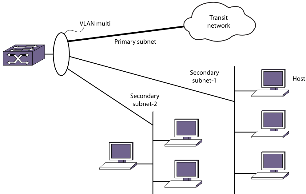
Figure 181: Multinetted Network Topology
