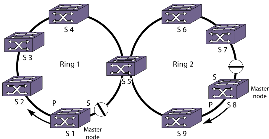
Figure 94: Two Rings Interconnected by One Switch
