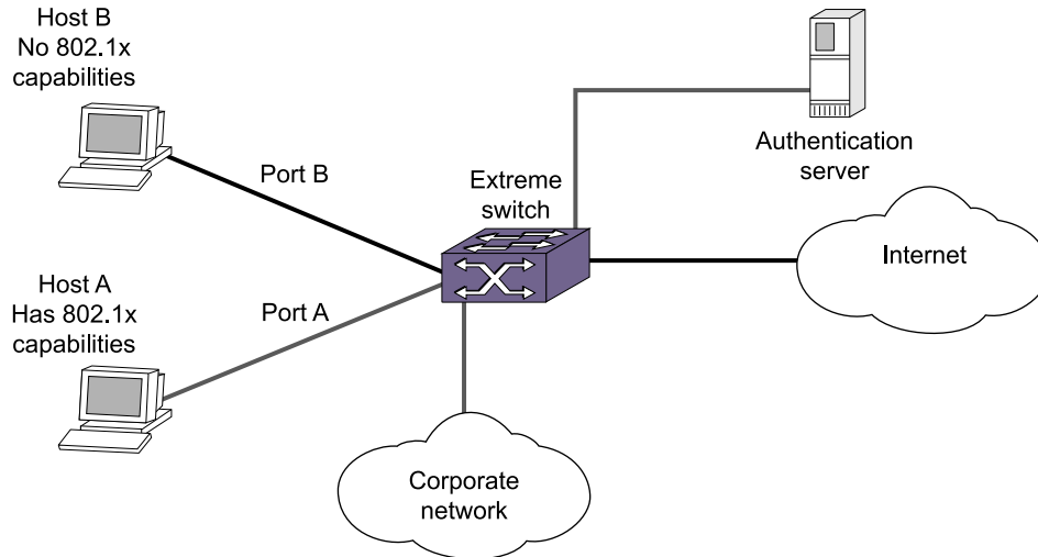
Figure 84: Guest VLAN for Network Login
