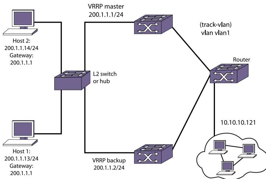
Figure 154: VRRP Tracking
