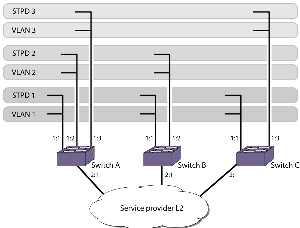
Figure 120: Sample Network Using STPD BPDUs Tunneling
