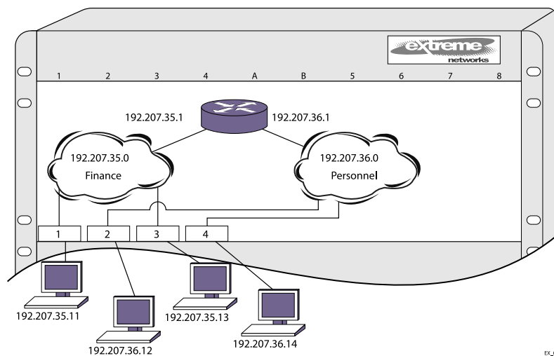
Figure 177: Routing Between VLANs
