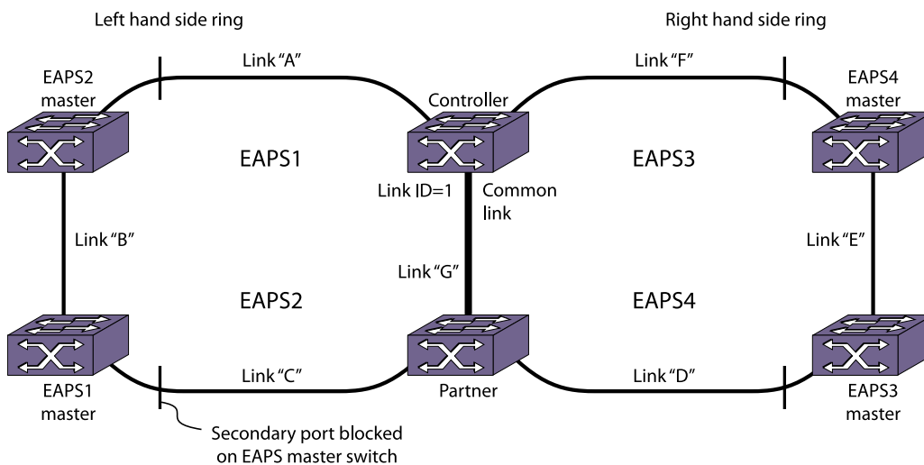
Figure 102: EAPS Common Link Topology with Spatial Reuse
