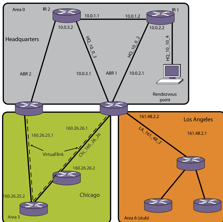
Figure 217: IP Multicast Routing Using PIM-SM Configuration Example
