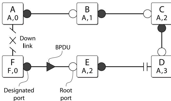
Figure 129: Down Link Detected
