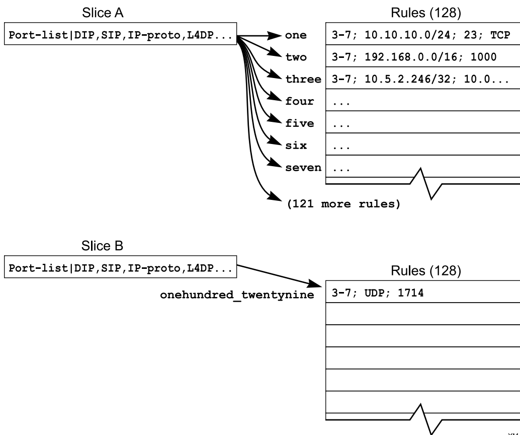
Figure 79: ACL Entry One Through onehundred_twentynine
