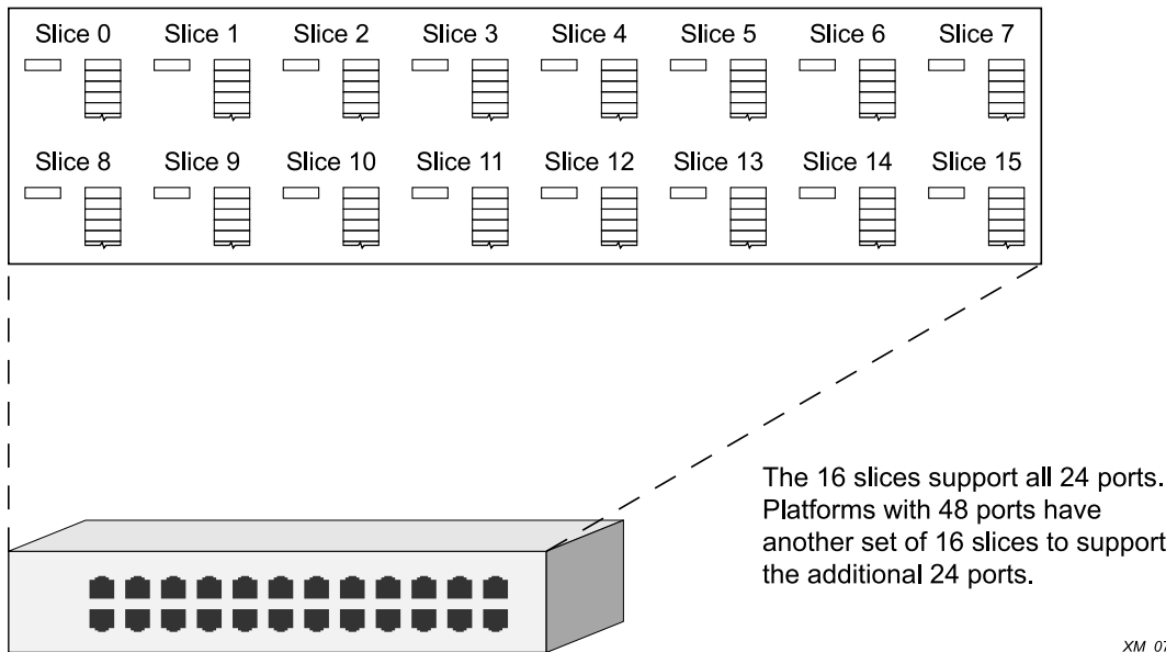
Figure 76: Slice Support for Summit X450a Series Switches and BlackDiamond 8800 a-Series Modules
