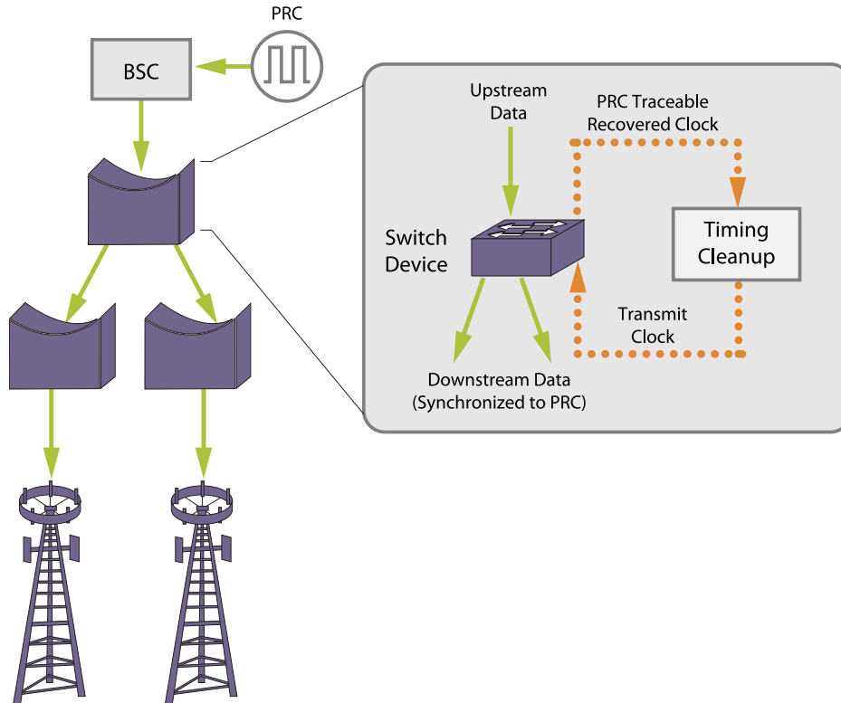
Figure 10: SyncE Structure
