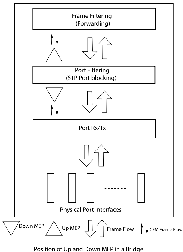
Figure 38: CFM UP and DOWN MEP at the Logical Level
