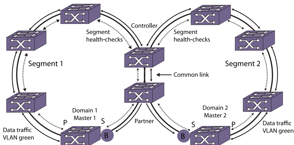
Figure 97: Segment Health-Check Messages
