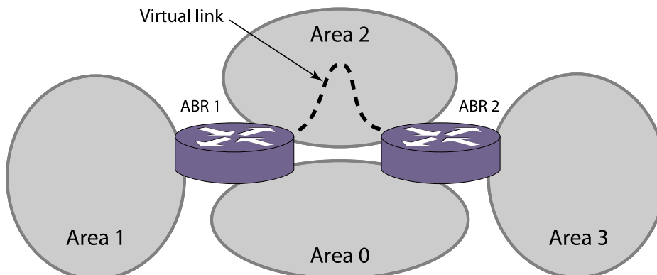
Figure 195: Virtual Link Providing Redundancy
