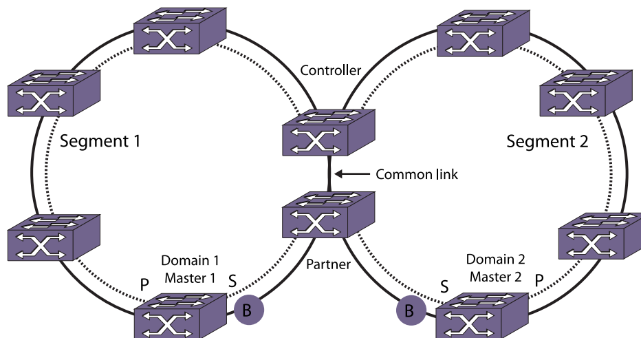
Figure 96: Master Node Operation in a Multiple Ring Topology
