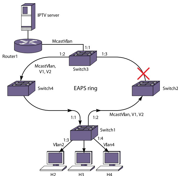
Figure 223: MVR on an EAPS Ring
