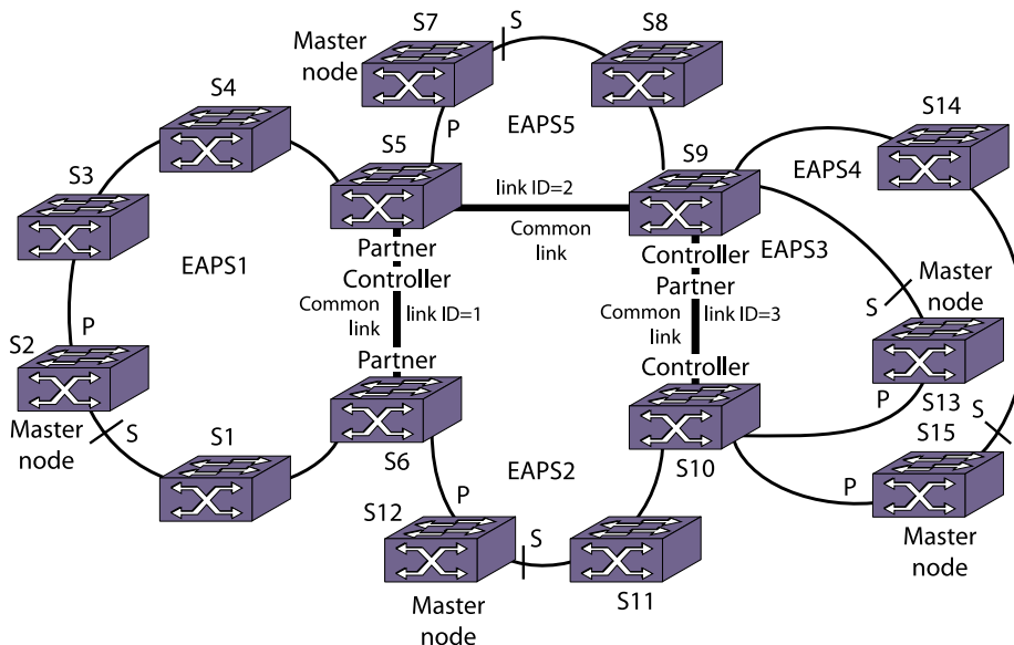
Figure 105: Basic Core and Right Angle Topology
