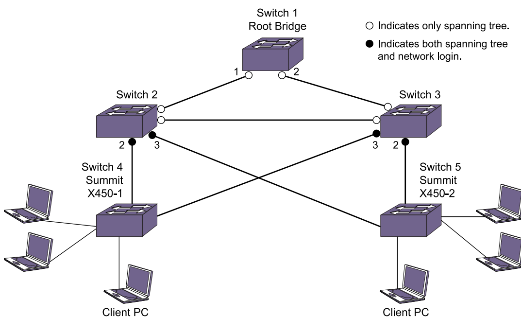
Figure 140: STP and Network Login Enabled
