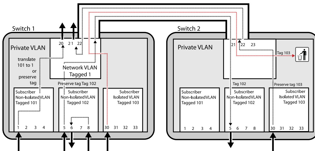
Figure 58: Private VLAN Support on Multiple Switches
