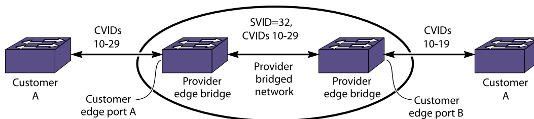
Figure 70: CVID Egress Filtering
