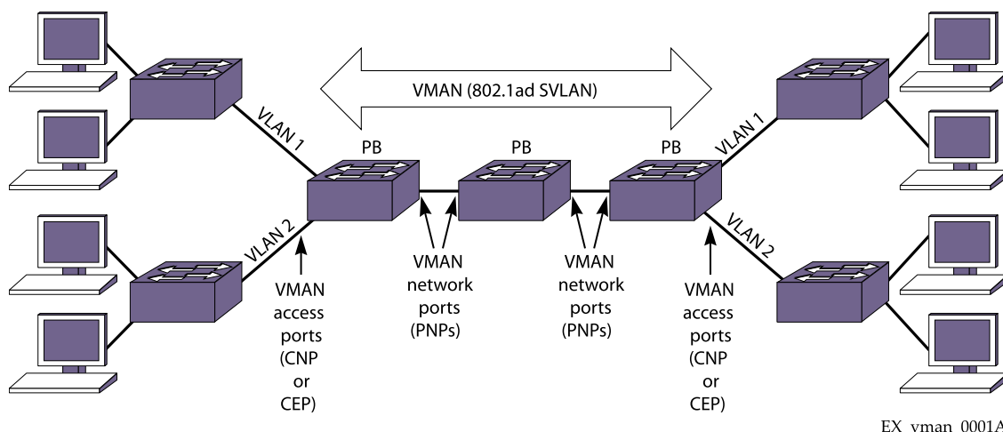
Figure 66: VMAN
