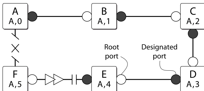
Figure 134: Completing the Topology Change
