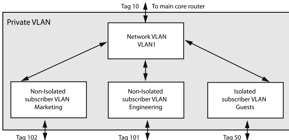
Figure 57: Private VLAN Switch Components
