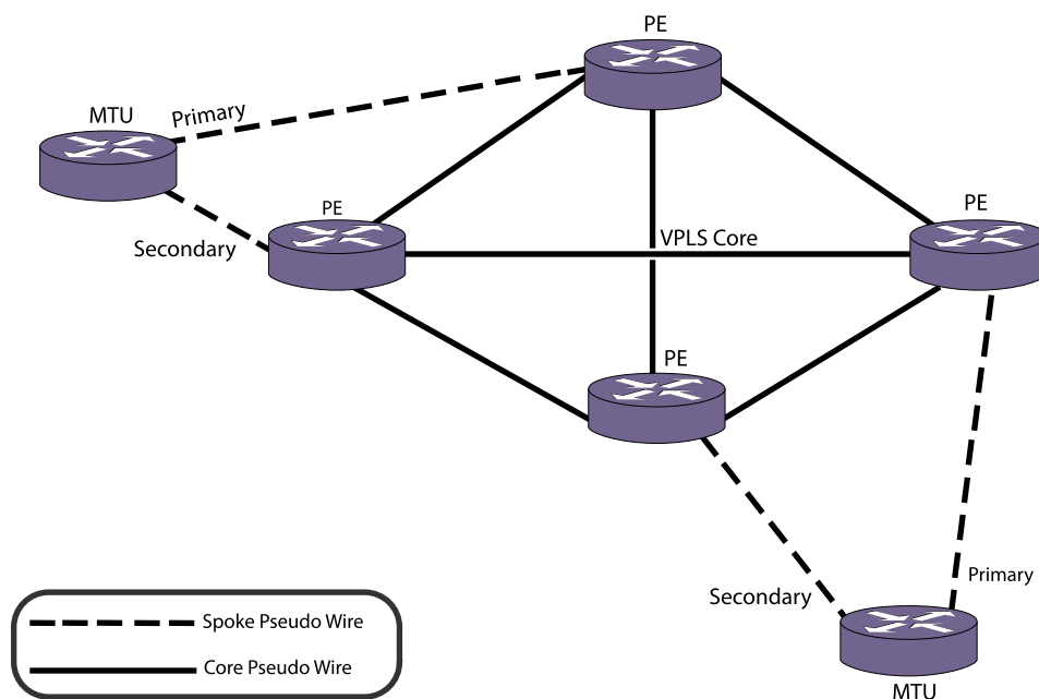
Figure 162: Example H-VPLS Network with Redundant Spokes
