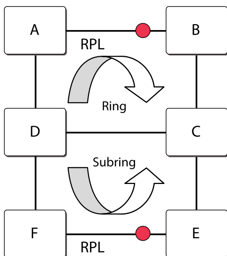
Figure 117: Ring and Sub-ring Network
