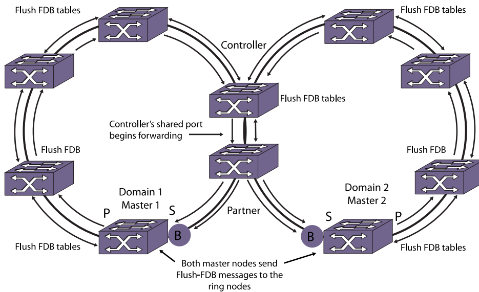
Figure 101: Common-Link Restored
