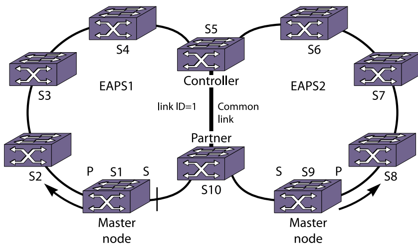
Figure 95: Multiple Rings Sharing a Common Link
