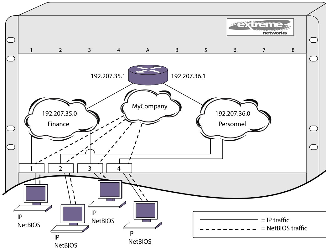
Figure 187: RIP Configuration Example
