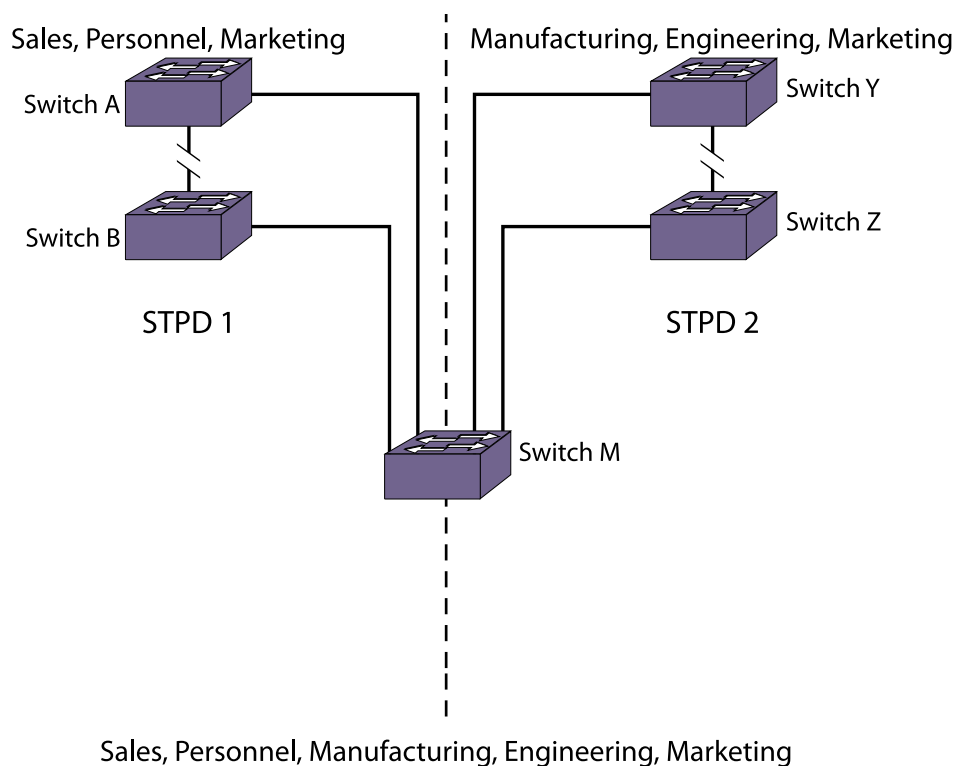
Figure 121: Multiple STPDs
