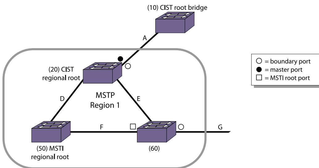
Figure 137: Close-Up of MSTP Region 1
