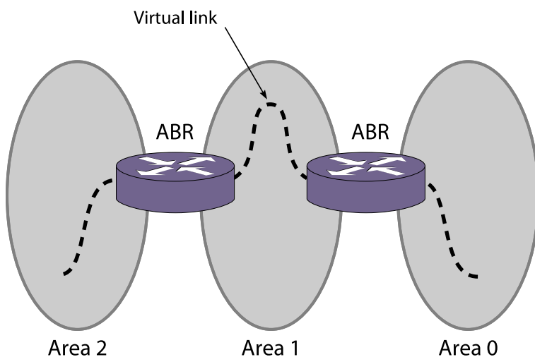
Figure 190: Virtual Link Using Area1 as a Transit Area
