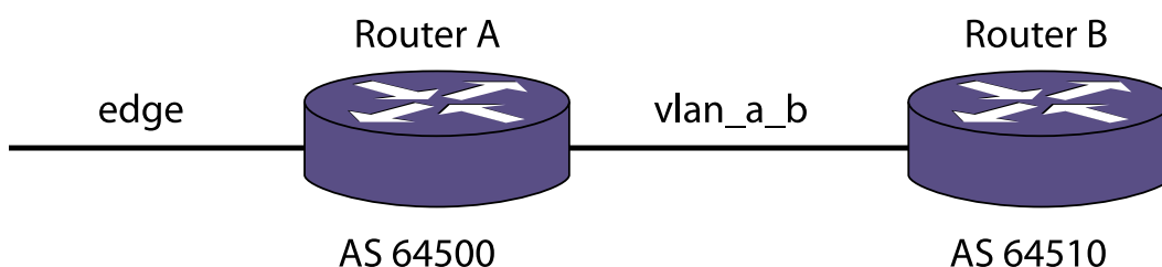
Figure 207: BGP IPv4 Route Filtering Example
