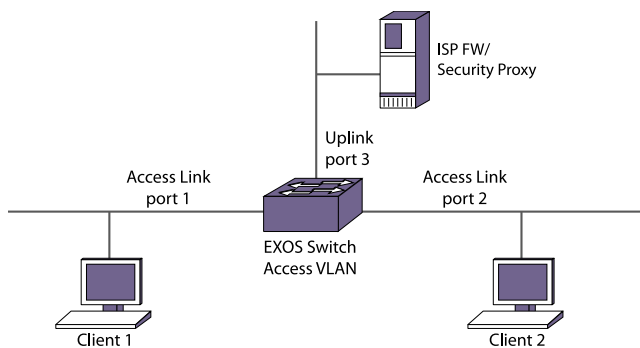
Figure 73: Upstream Forwarding or Disabling Egress Flooding Example
