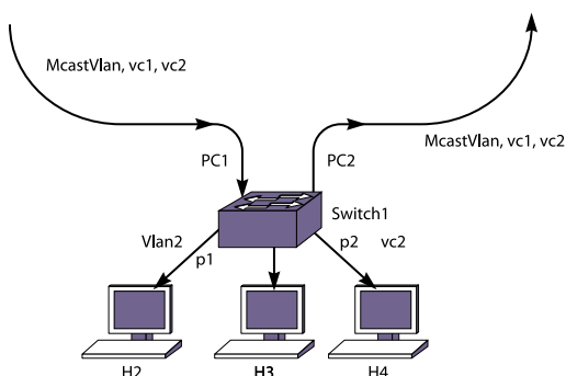
Figure 221: Multiple VLANs in the Core Network
