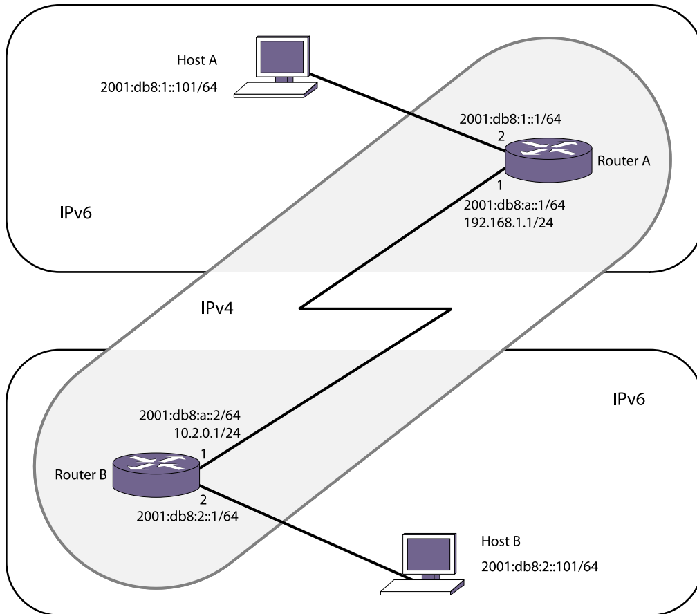
Figure 184: 6in4 Tunnel Example
