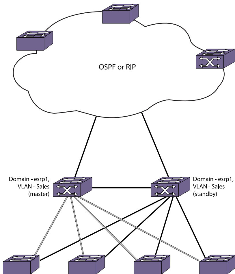
Figure 149: Single ESRP Domain Using Layer 2 and Layer 3 Redundancy
