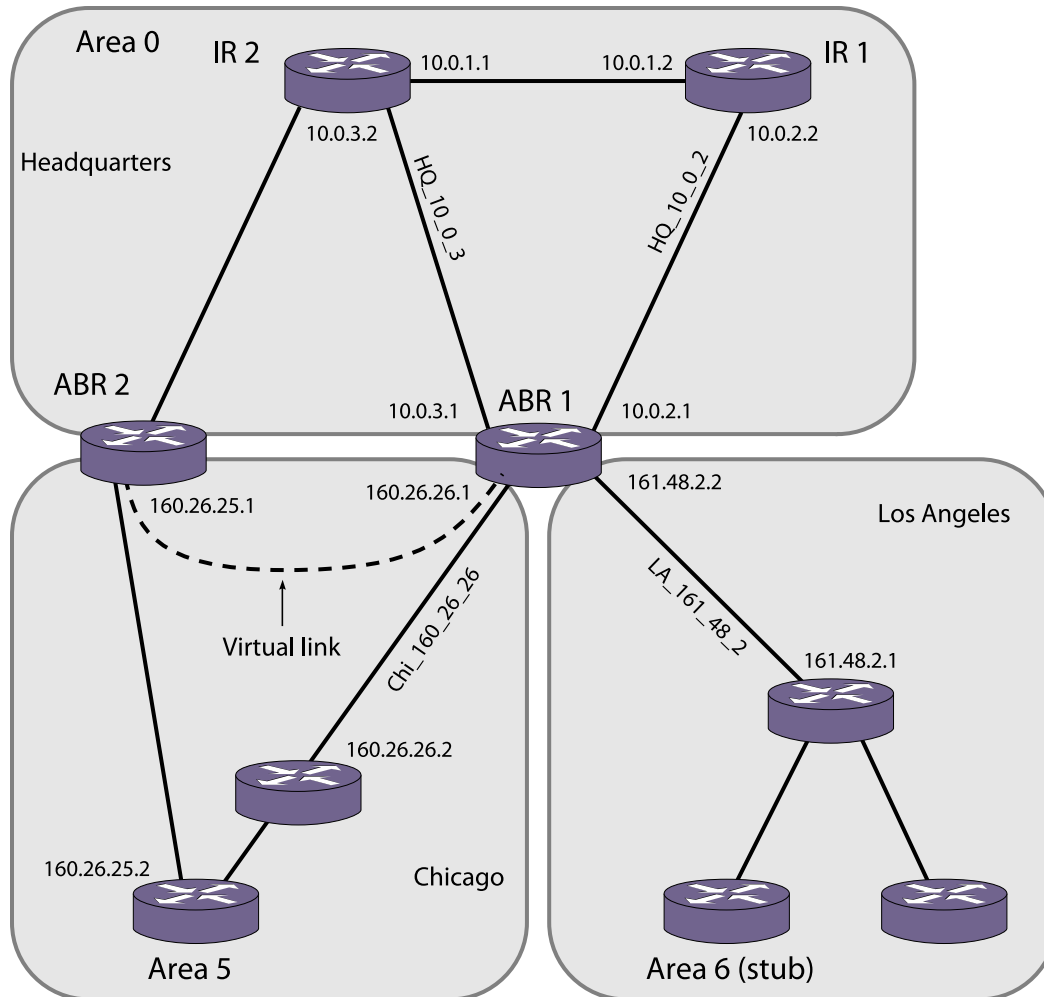
Figure 193: OSPF Configuration Example
