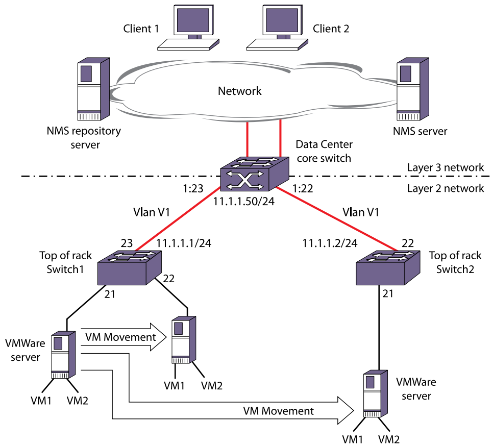
Figure 74: Sample XNV Topology
