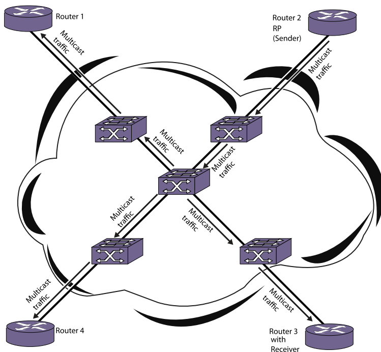
Figure 214: Multicast Without PIM Snooping
