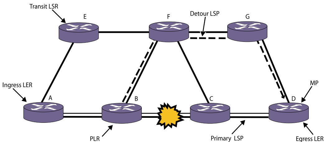
Figure 170: Fast-Reroute Terminology
