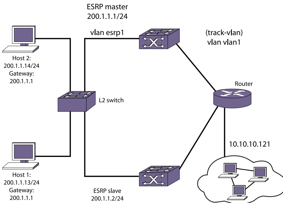
Figure 147: ESRP Tracking
