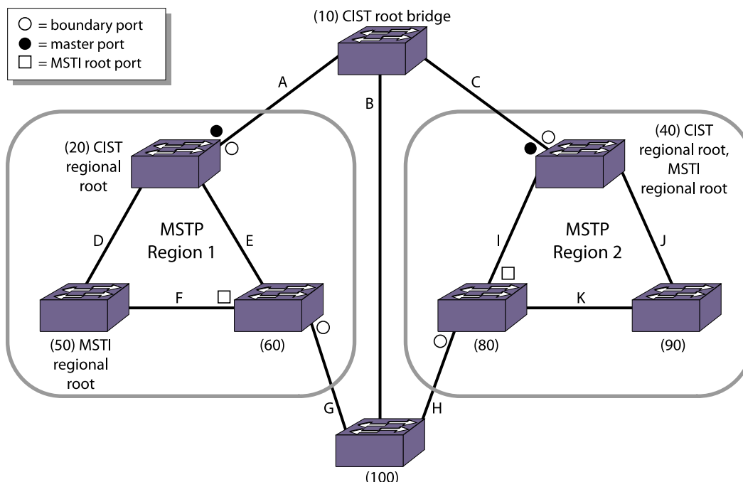
Figure 136: Sample MSTP Topology with Two MSTP Regions
