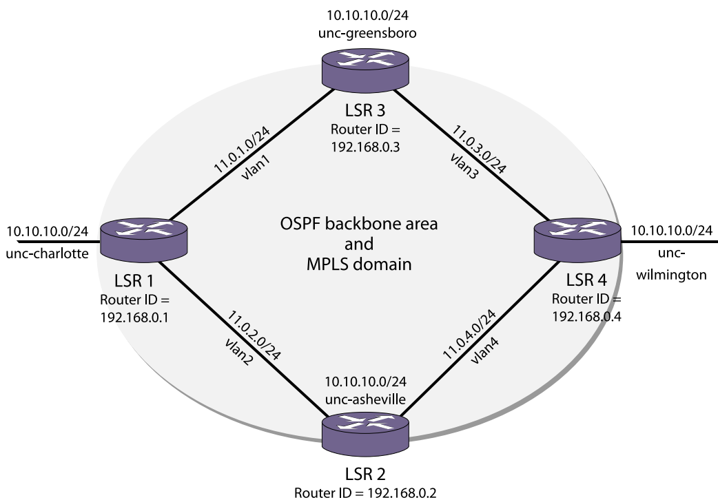
Figure 175: Full Mesh Configuration Example
