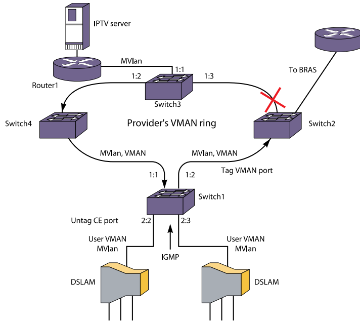
Figure 225: MVR in a VMAN Environment
