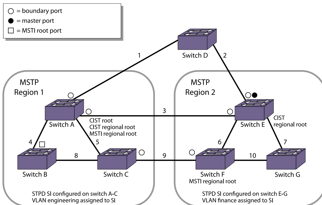
Figure 139: MSTP Topology with the CIST Root Bridge Contained within a Region
