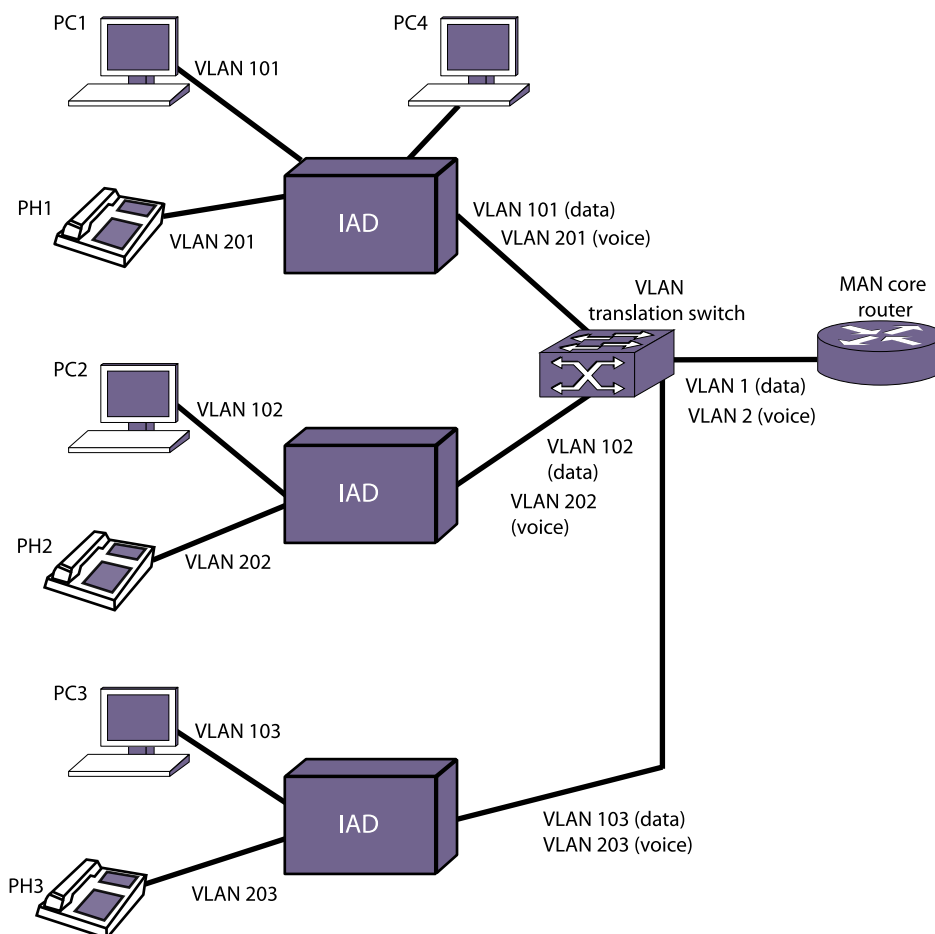
Figure 55: VLAN Translation Application
