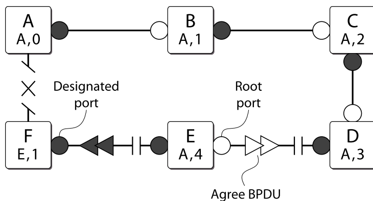
Figure 133: Communicating Port Status to Neighbors
