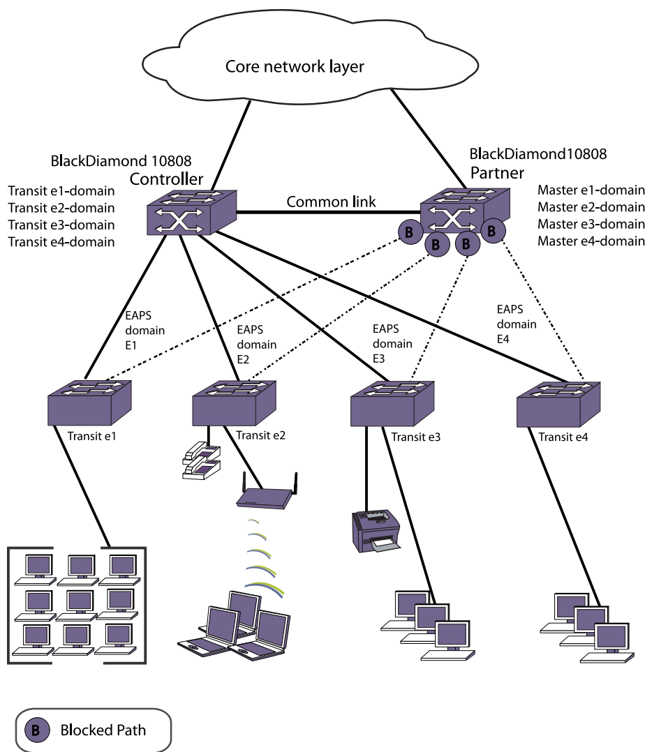
Figure 111: L2 Aggregation Network Layer
