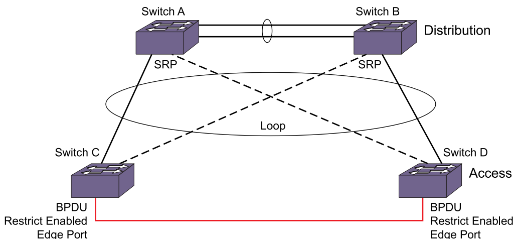
Figure 119: BPDU Restrict
