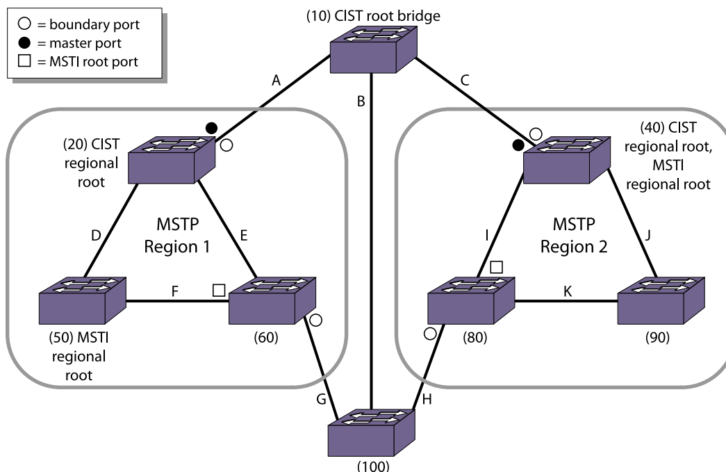
Figure 138: Sample MSTP Topology with Two MSTP Regions
