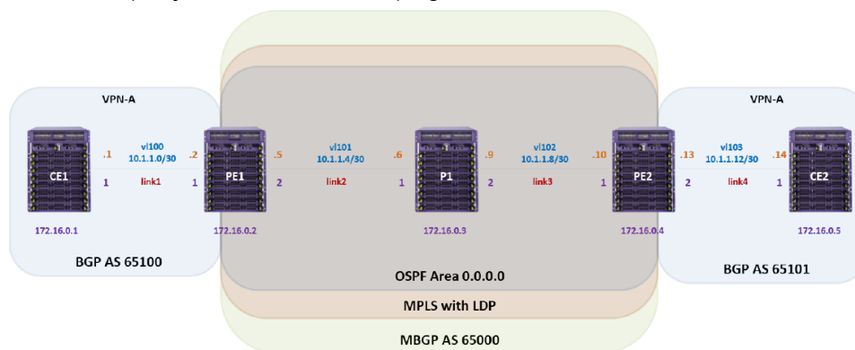
Figure 212: Layer 3 Virtual Private Network
