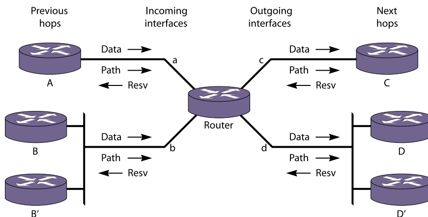
Figure 169: RSVP Messages
