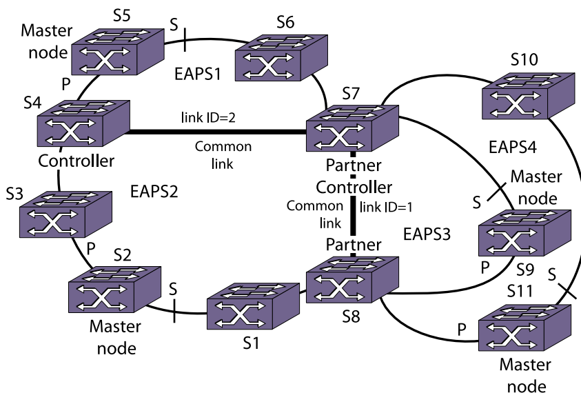
Figure 104: Right Angle Topology
