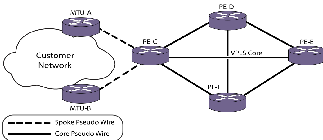
Figure 164: Example Protected Access H-VPLS Network
