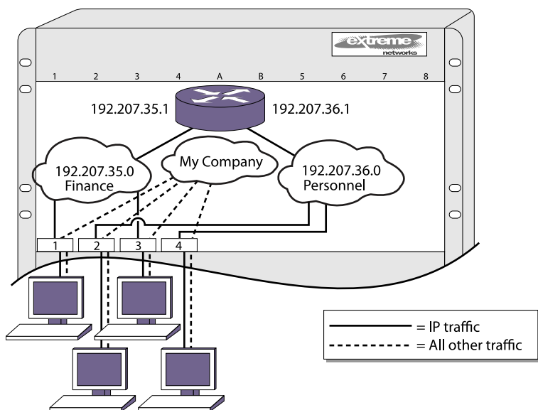
Figure 54: Protocol-Based VLANs
