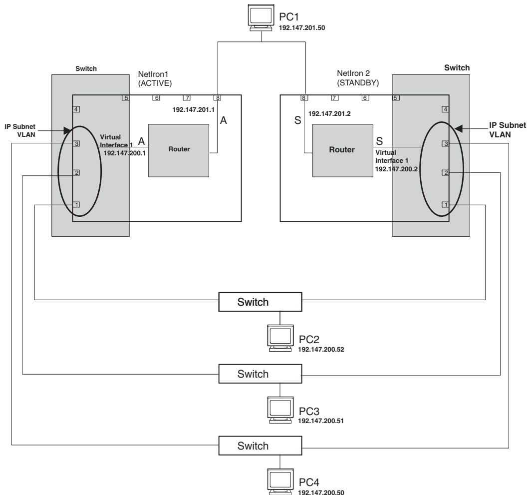
Figure 14.6 Configuring FSRP on virtual interfaces
