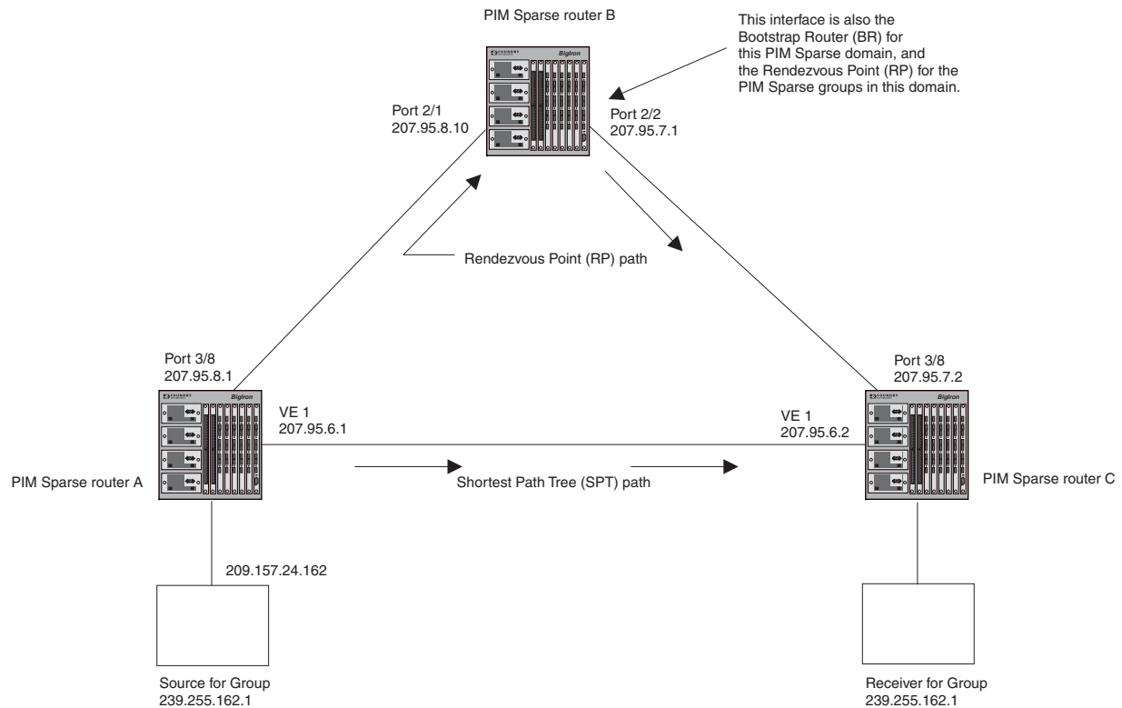
Figure 8.3 Example PIM Sparse domain
