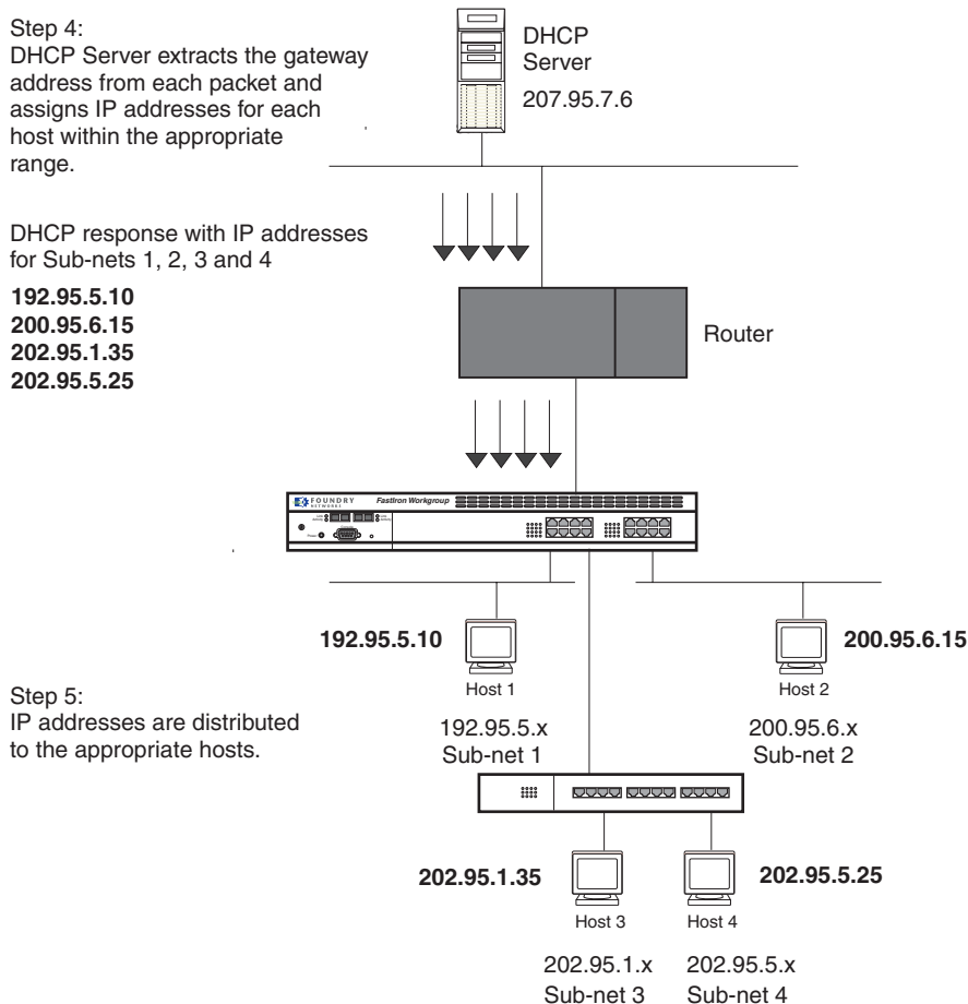
Figure 6.12 DHCP offers are forwarded back toward the requestors
