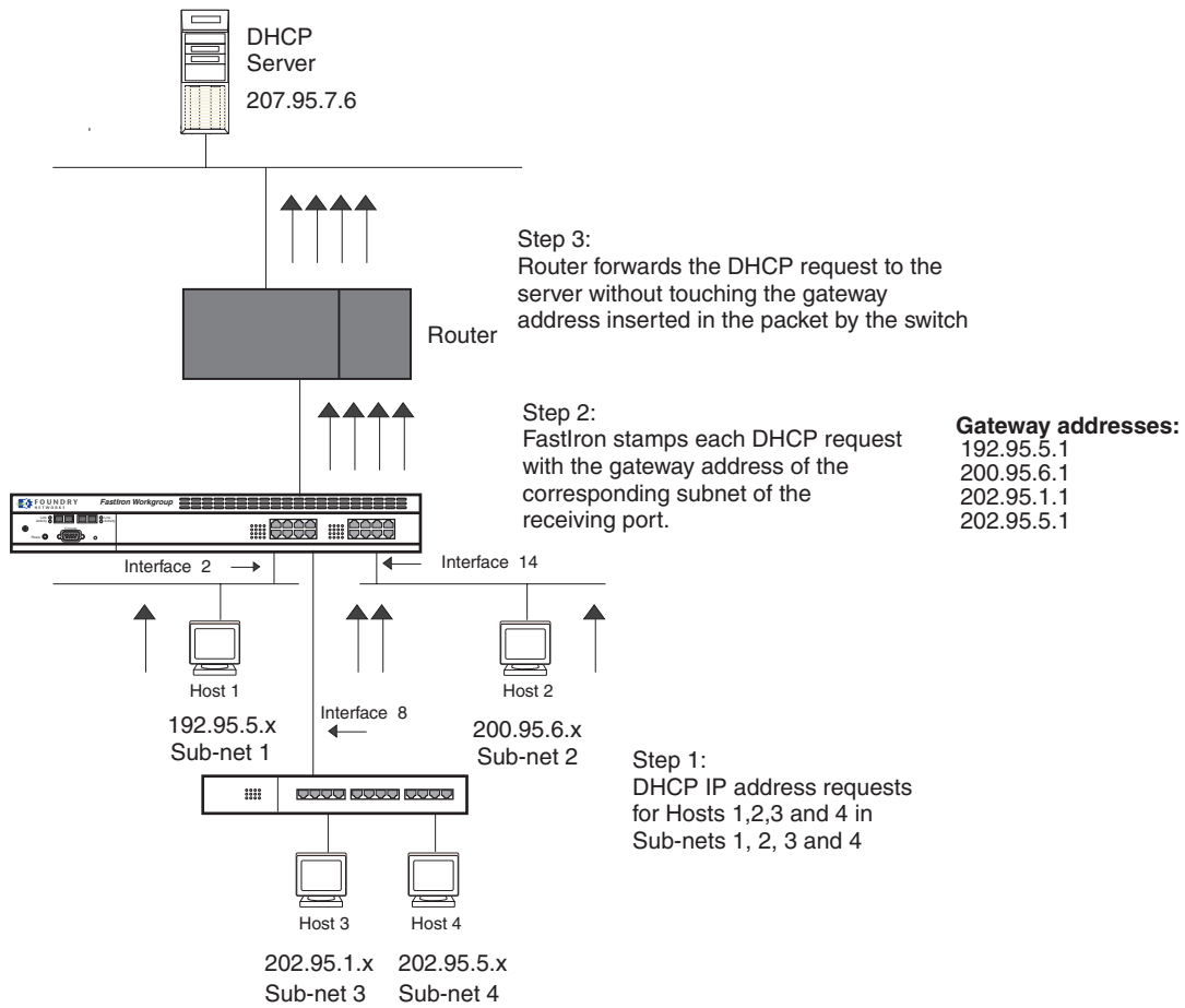
Figure 6.11 DHCP requests in a network with DHCP Assist operating on a FastIron
