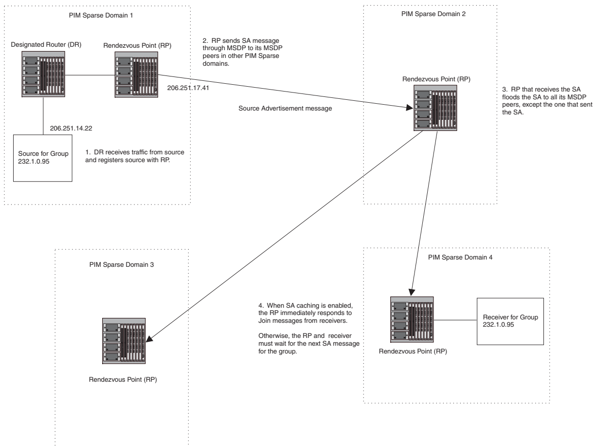
Figure 8.4 PIM Sparse domains joined by MSDP routers
