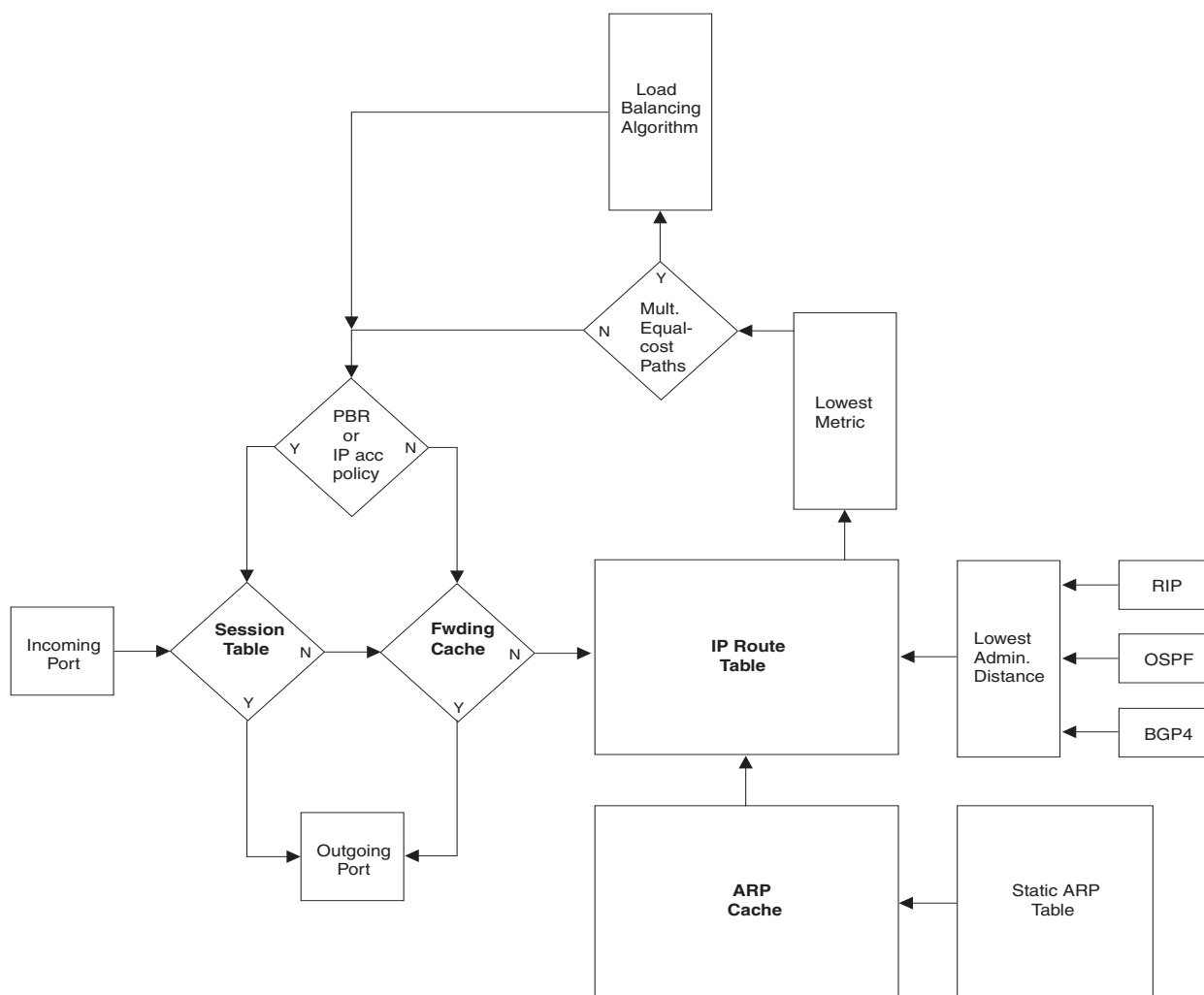
Figure 6.1 IP Packet flow through a Foundry Layer 3 Switch
