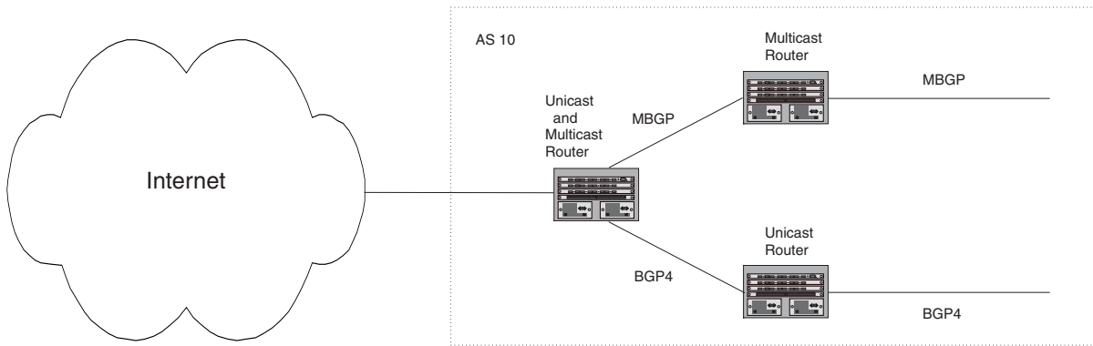
Figure 11.1 MBGP used when multicast topology is different from unicast topology
