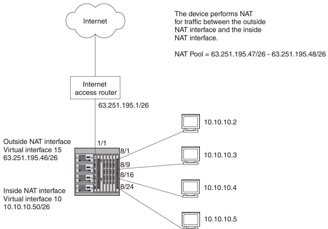
Figure 12.3 NAT clients connected directly to the Layer 3 Switch
