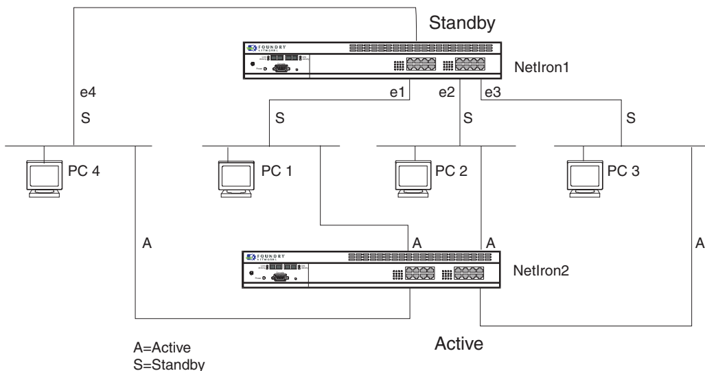
Figure 14.4 NetIron2 becomes active router after links e1 and e3 fail with multiple track ports defined
