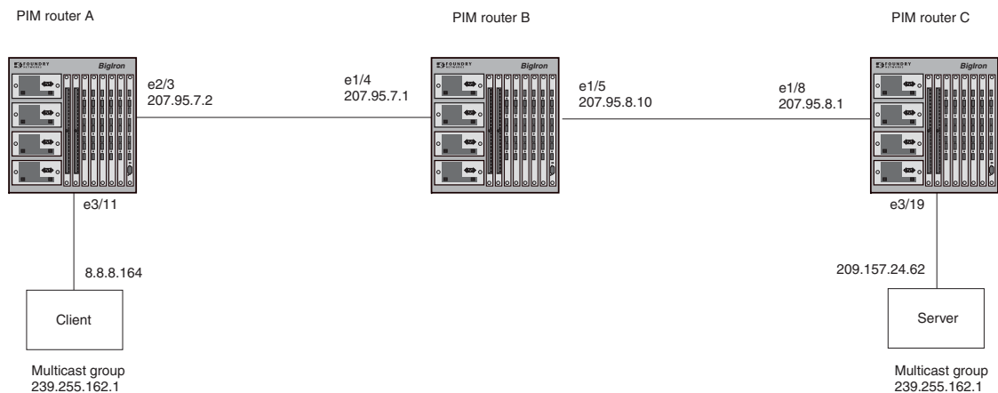
Figure 8.9 Example PIM Group
