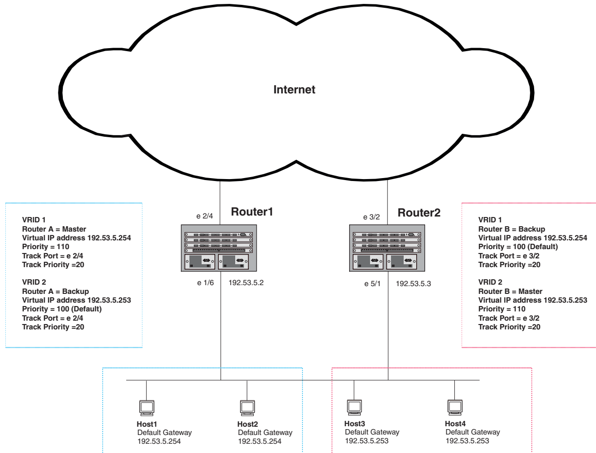
Figure 13.3 Router1 and Router2 are configured to provide dual redundant network access for the host
