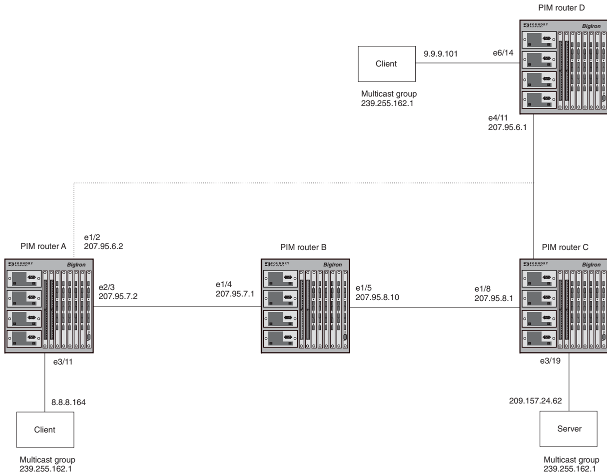
Figure 8.8 Example multicast static routes
