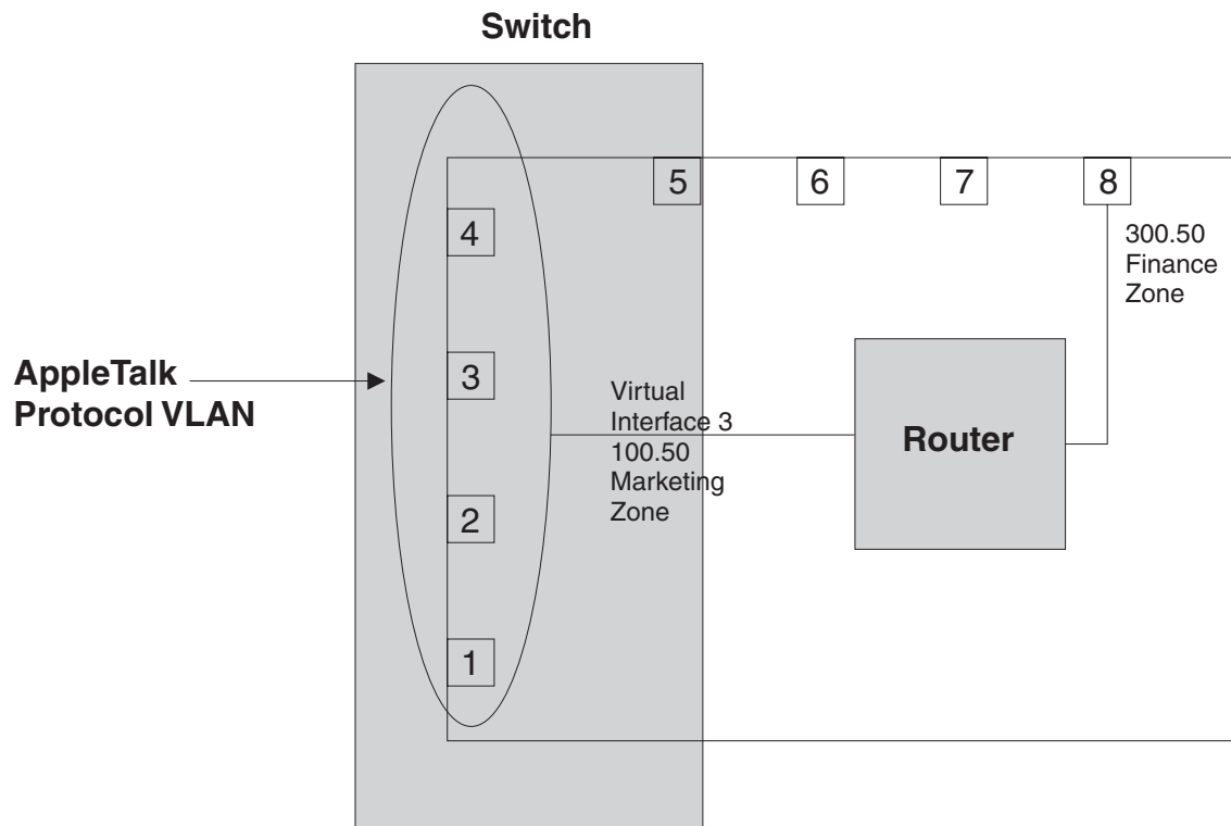
Figure 16.3 Virtual interface provides a routing interface to an AppleTalk VLAN
