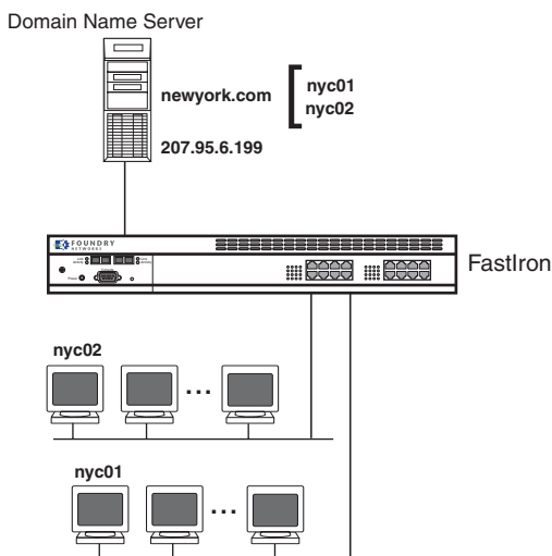
Figure 6.9 Querying a host on the newyork.com domain
