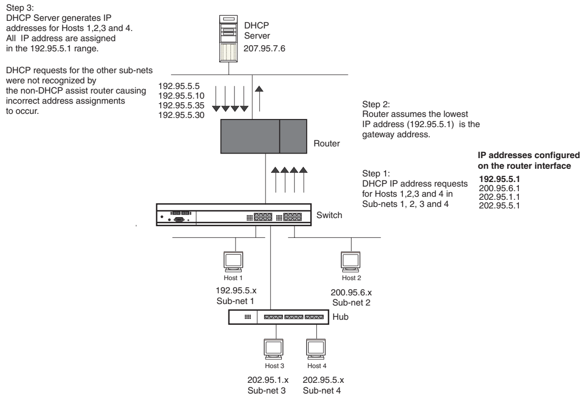
Figure 6.10 DHCP requests in a network without DHCP Assist on the Layer 2 Switch
