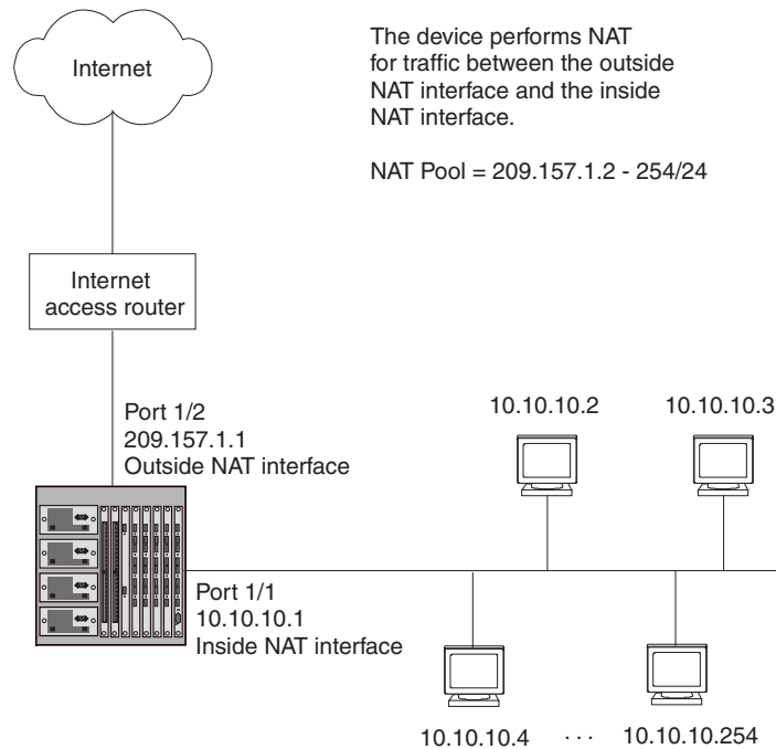
Figure 12.1 Network Using Inside NAT
