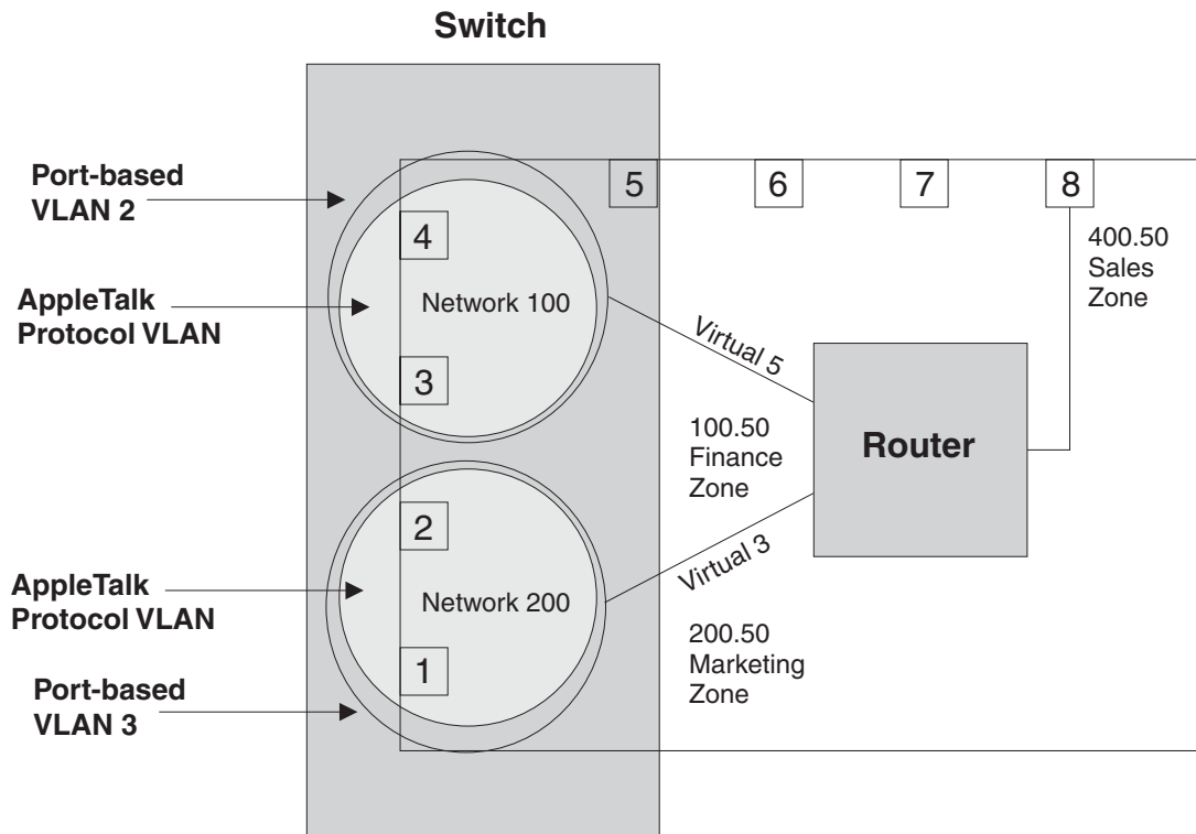
Figure 16.4 Routing between AppleTalk VLANs
