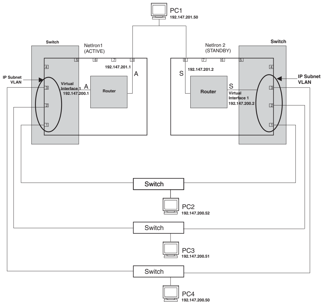
Figure 14.2 Virtual interface providing a redundant link
