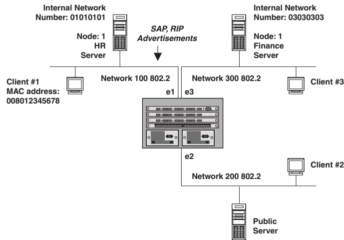
Figure 15.1 Defining and assigning IPX Forward, RIP and SAP filters
