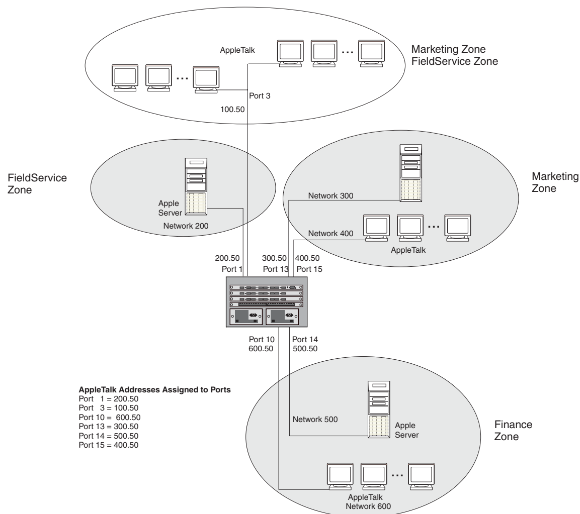
Figure 16.2 AppleTalk zones in a network
