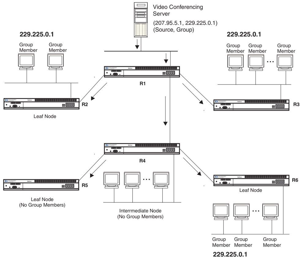
Figure 8.1 Transmission of multicast packets from the source to host group members
