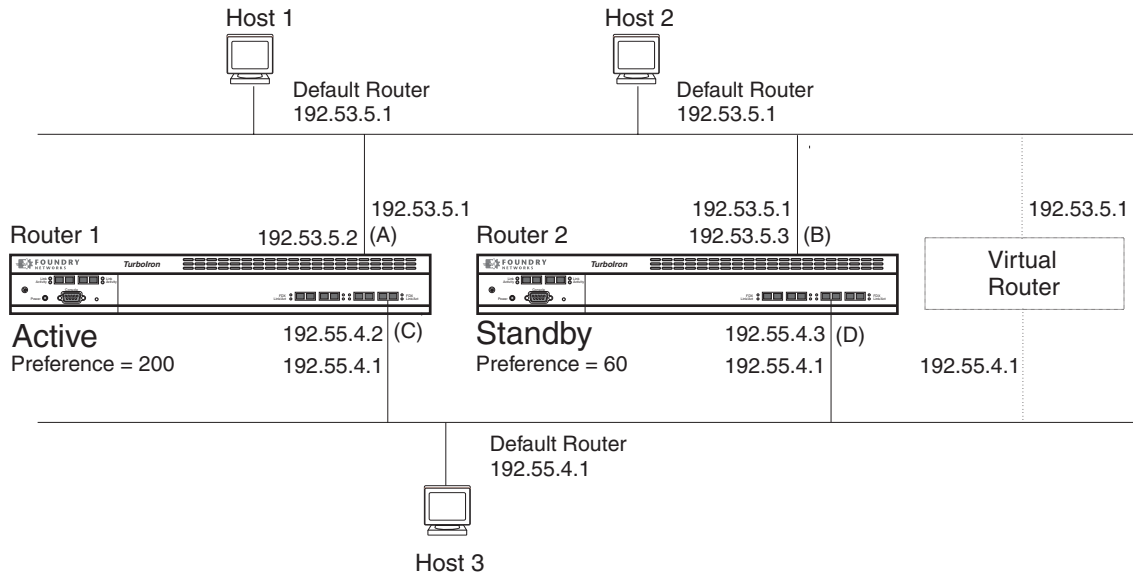
Figure 14.1 FSRP operating in a NetTron network
