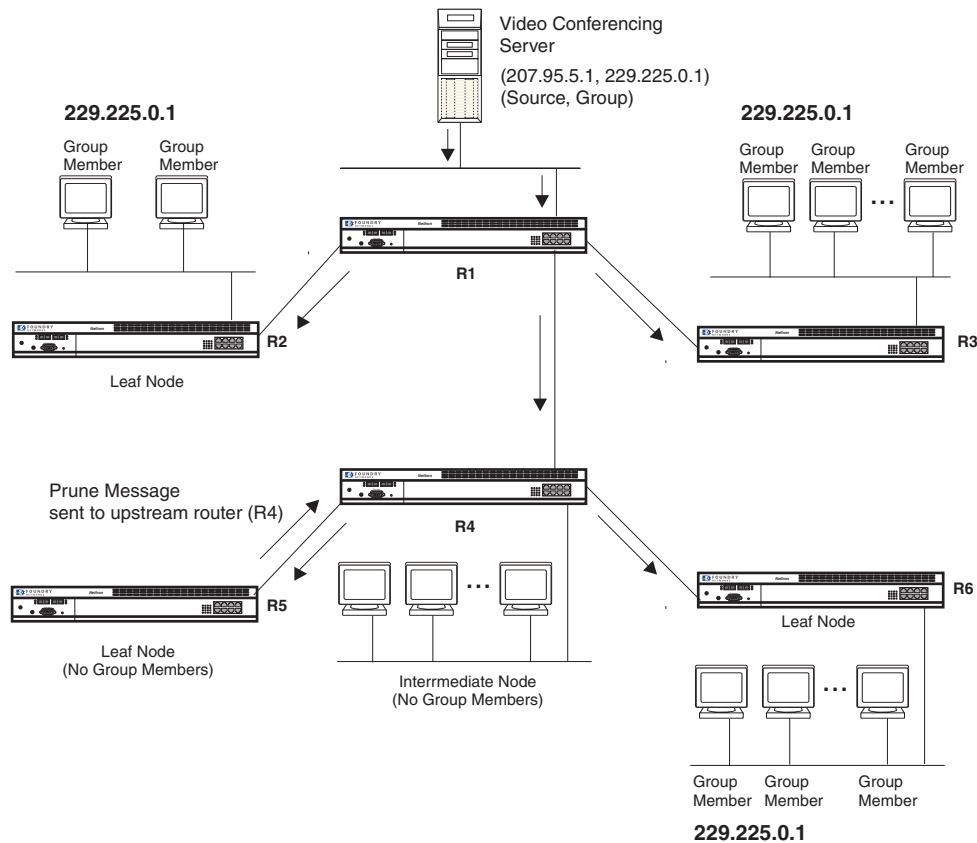
Figure 8.6 Pruning leaf nodes from a multicast tree
