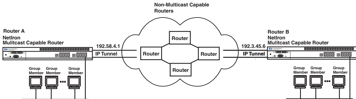
Figure 8.7 IP in IP tunneling on multicast packets in a unicast network
