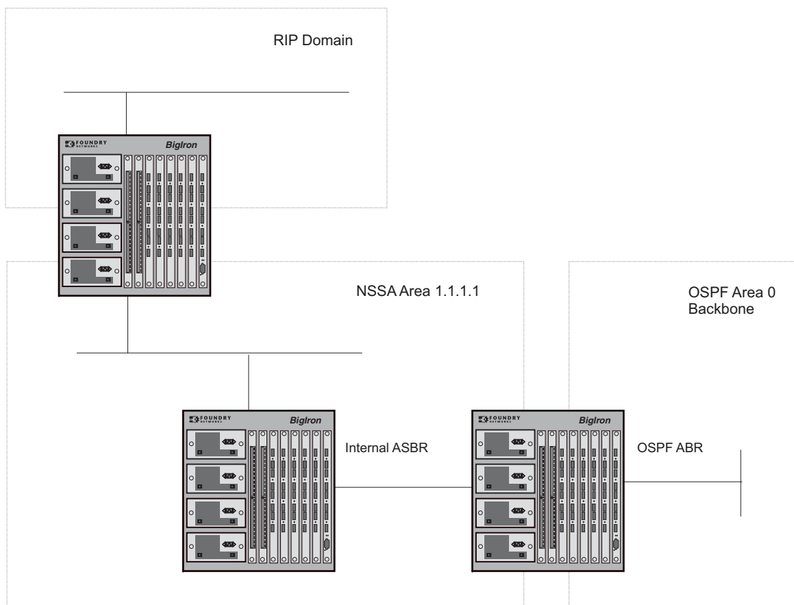
Figure 9.5 OSPF network containing an NSSA
