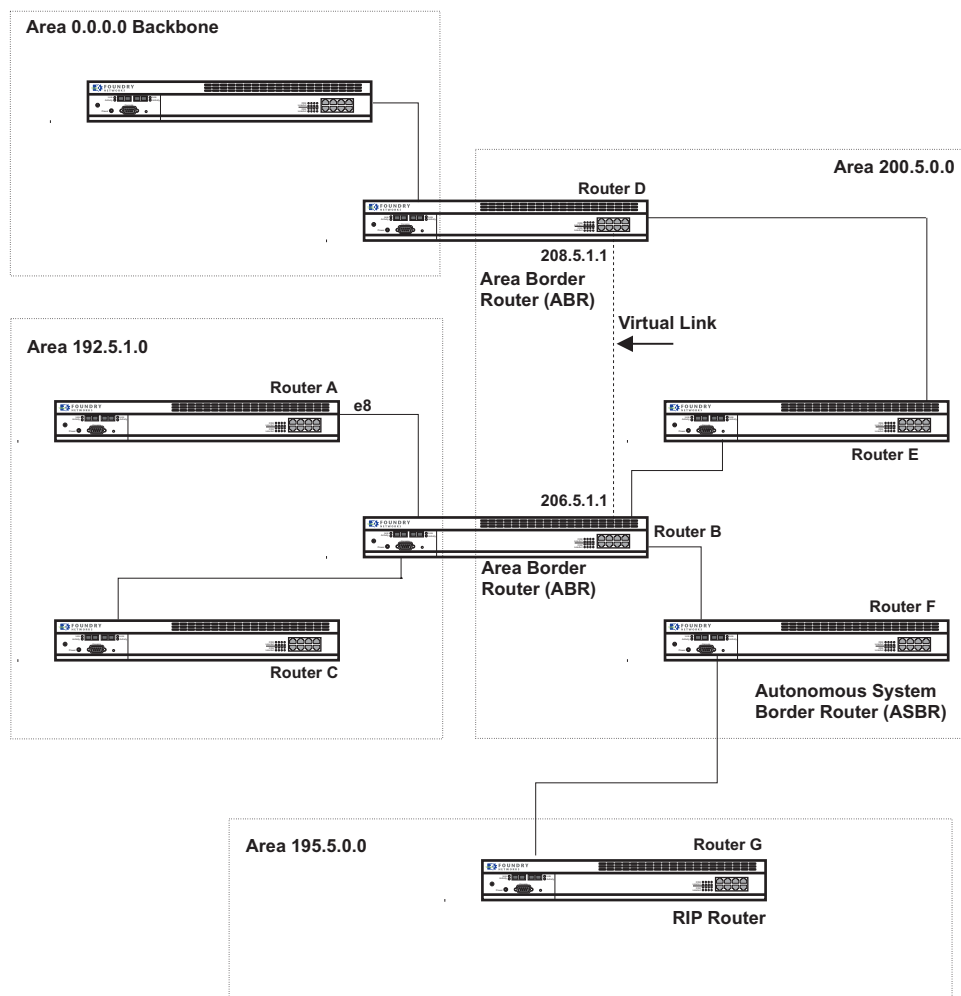
Figure 9.1 OSPF operating in a network
