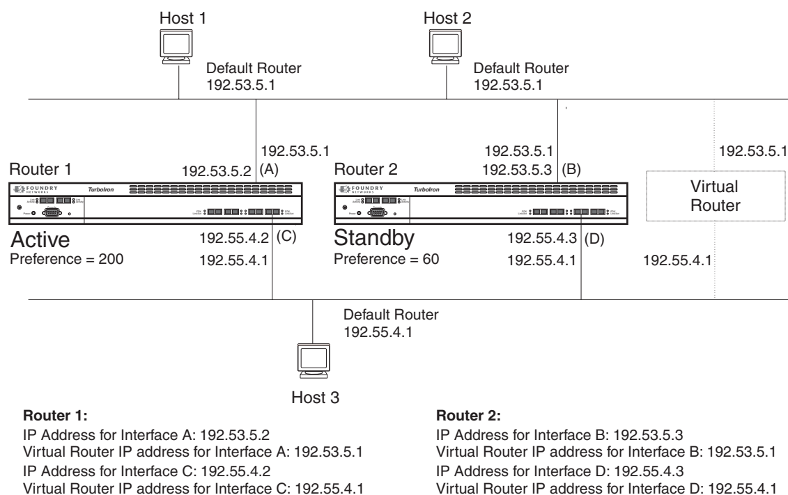
Figure 14.5 FSRP operating in a Netron network
