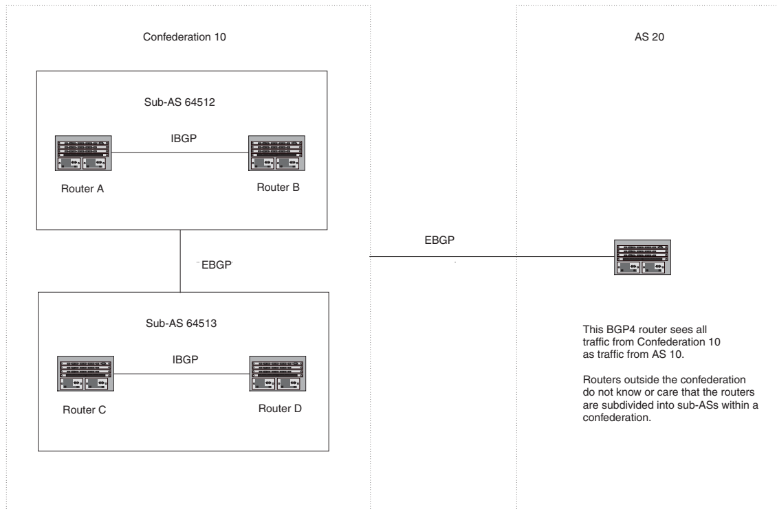
Figure 10.4 Example BGP4 confederation
