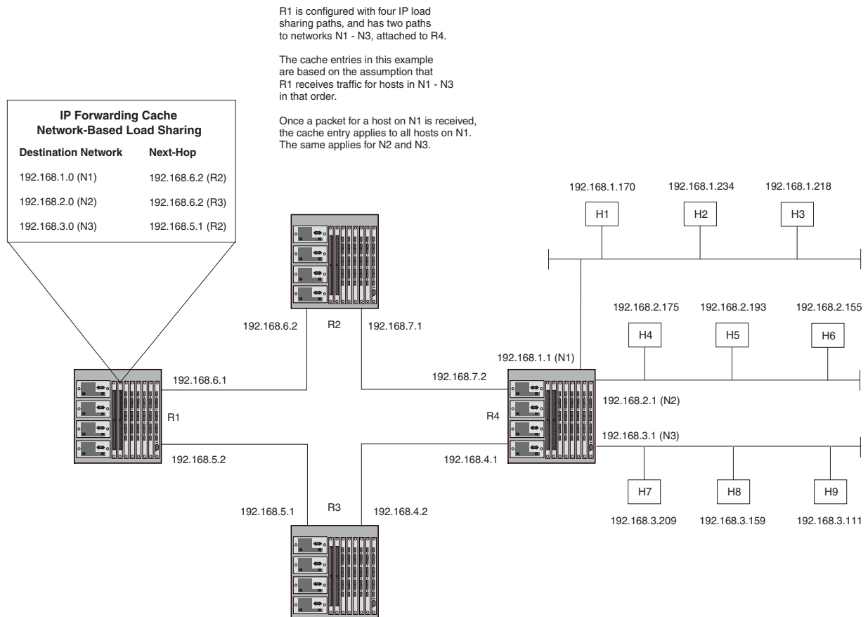
Figure 6.7 Network-based IP load sharing – basic example
