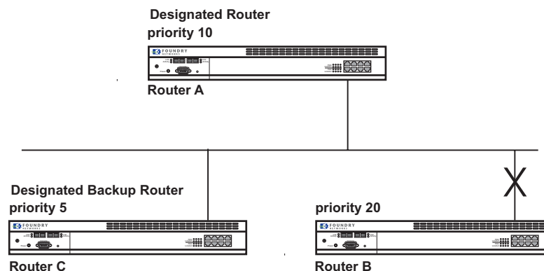
Figure 9.3 Backup designated router becomes a designated router
