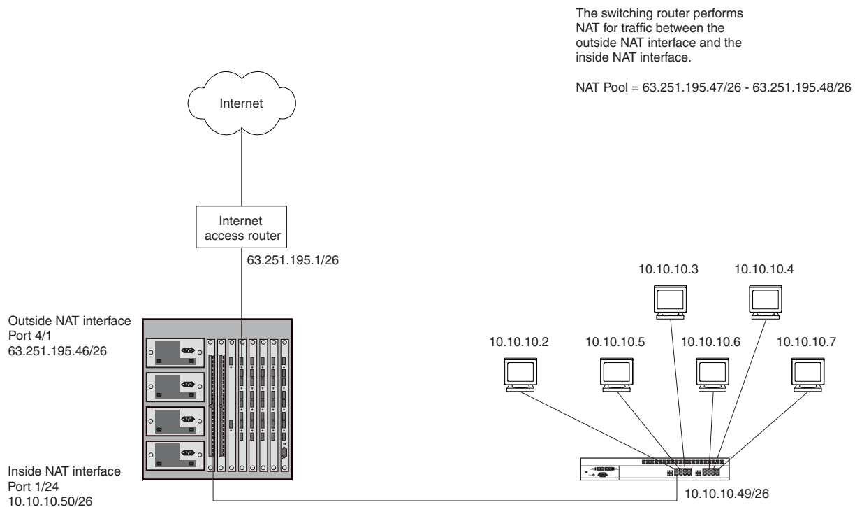
Figure 12.2 NAT clients connected the Layer 3 Switch by a Switch
