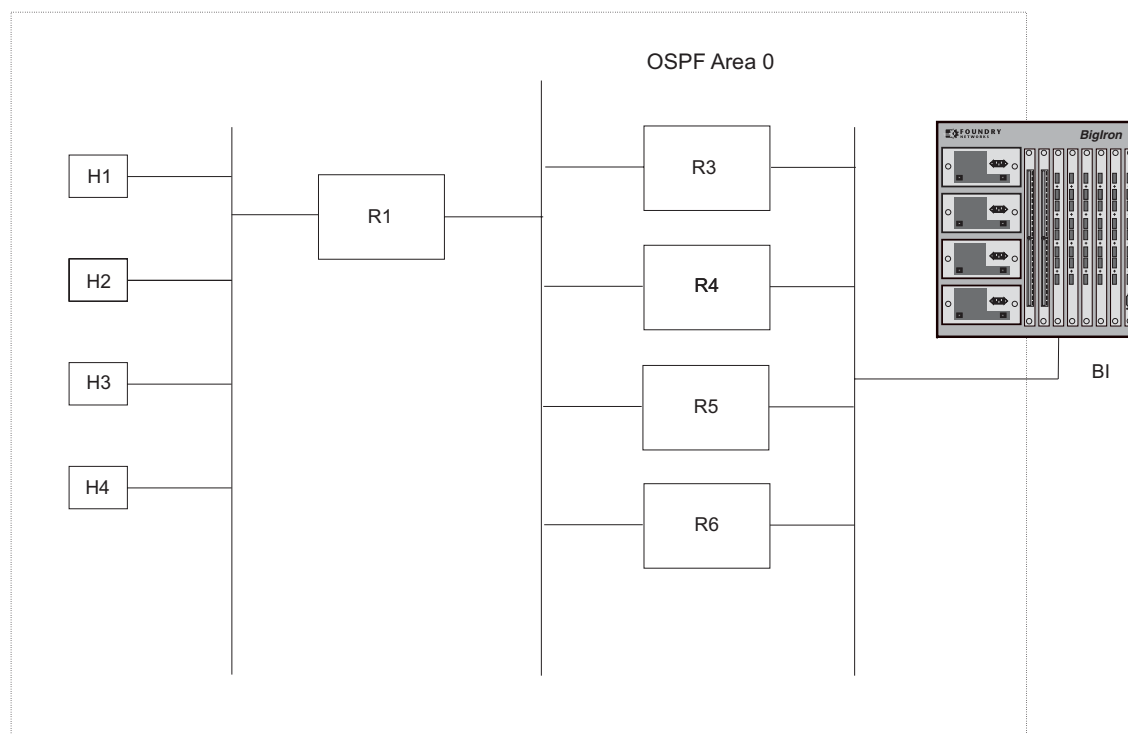
Figure 9.8 Example OSPF network with four equal-cost paths
