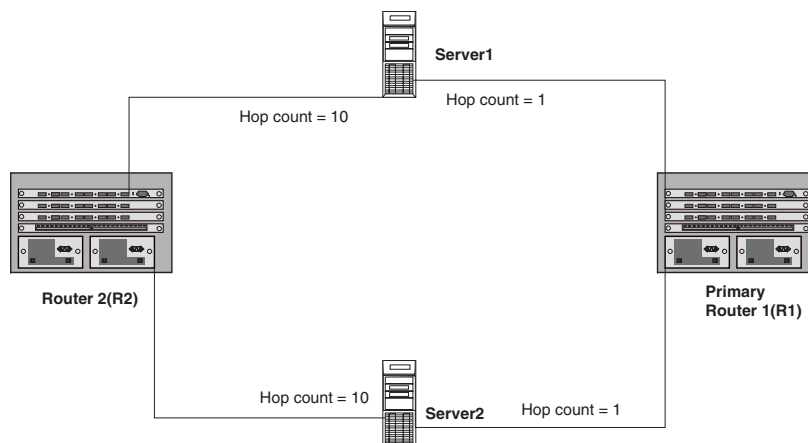
Figure 15.2 Using higher hop count assignments to bias traffic away from the router
